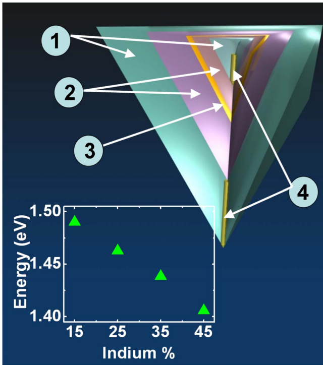
FIG. 1. (Color online) An illustration of the sample layer structure following the etch-stop layer used to facilitate substrate removal. Label 1—Al 0.55 Ga 0.45 As layer, 2—GaAs barriers, 3—In x Ga 1-x As dot layer, and 4—vertical quantum wire. Inset: emission energy tuning as a function of indium percentage in the QD composition.
