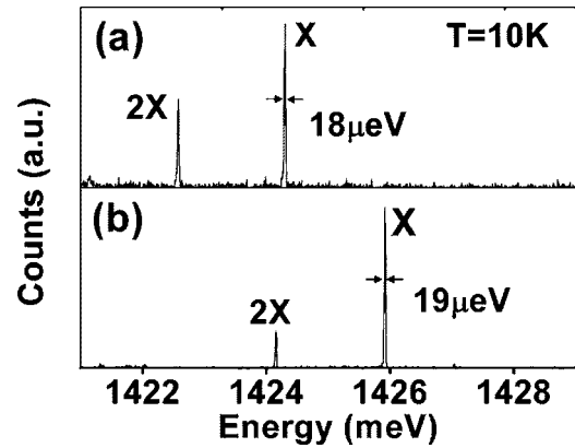
FIG. 3. ( \mu PL) spectra taken from two different individual QDs. Emission from the neutral exciton (X) and biexciton (2X) states is labeled. The width of the neutral exciton peaks were extracted by fitting a Lorentzian peak. Integration times and excitation intensities are different for the two spectra.
