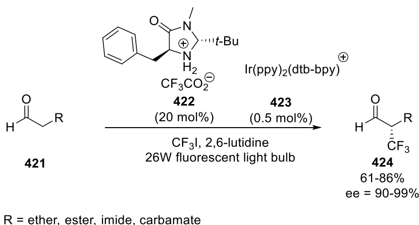
Scheme 7.47 Enantioselective trifluoromethylation of aldehydes using trifluoriodomethane as the trifluoromethyl source, amine catalyst 422 , Ir catalyst 423 and light.
