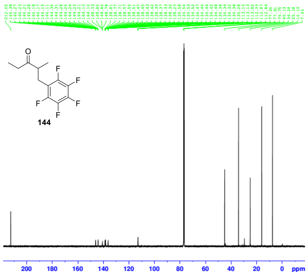
Figure 2.3 13 C NMR spectrum of 2-methyl-1-(perfluorophenyl)pentan-3-one 144 .
