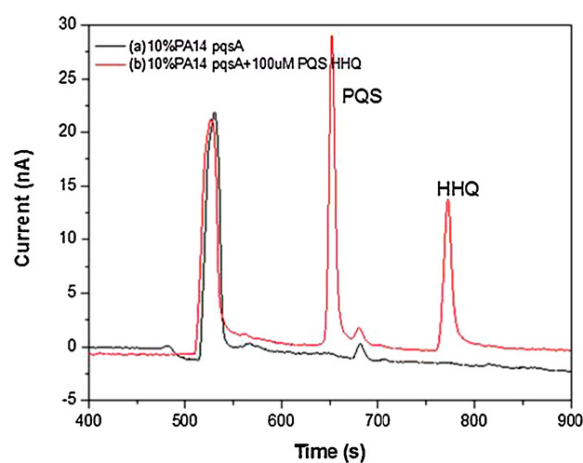
Fig. 6. Analysis of P. aeruginosa pqsA mutant strain using the PDDA coated capillary (50 \mu\text{m} id and 45 cm effective length). (a) pqsA mutant strains diluted 10-fold with the running buffer. (b) pqsA mutant strains diluted 10-fold with running buffer spiked with 100 \mu\text{M} standard (1) PQS and (2) HHQ. Running buffer, 50 mM \text{H}_3\text{PO}_4 -Tris, pH 2, 20% (v/v) ACN; separation voltage, -10 kV; injection time, 5 s at -10 kV; BDD electrode poised at +1.5 V vs. Ag/AgCl.
