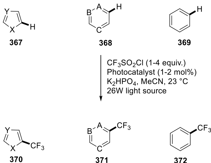
Scheme 8.2 Trifluoromethylation by means of a photoredox catalyst.
