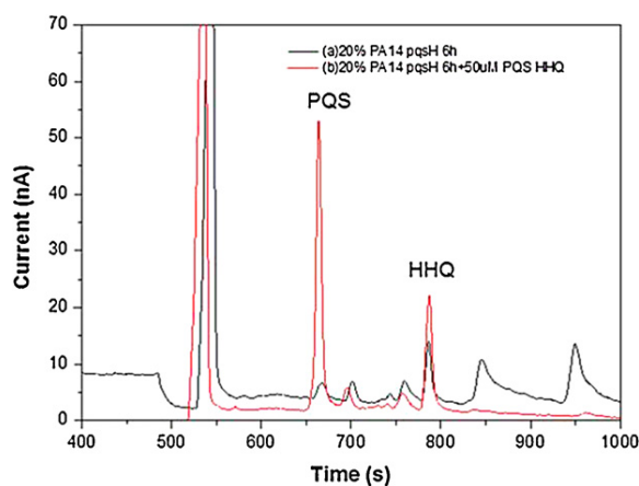
Fig. 7. Analysis of P. aeruginosa pqsH mutant strain using the PDPA coated capillary (50 \mu\text{m} id and 45 cm effective length). (a) pqsH mutant strains diluted 10-fold with the running buffer. (b) pqsH mutant strains diluted 10-fold with the running buffer spiked with 50 \mu\text{M} standard (1) PQS and (2) HHQ. Running buffer, 50 mM \text{H}_3\text{PO}_4 -Tris, pH 2, 20% (v/v) ACN; separation voltage, -10 kV; injection time, 5 s at -10 kV; BDD electrode poised at +1.5 V vs. Ag/AgCl.
