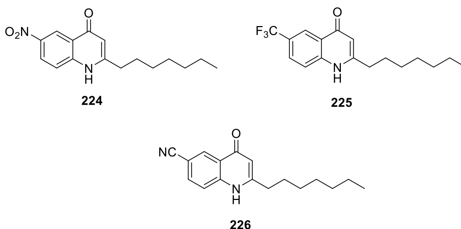
Figure 4.21 Analogues with electron-withdrawing groups present at C-6.
