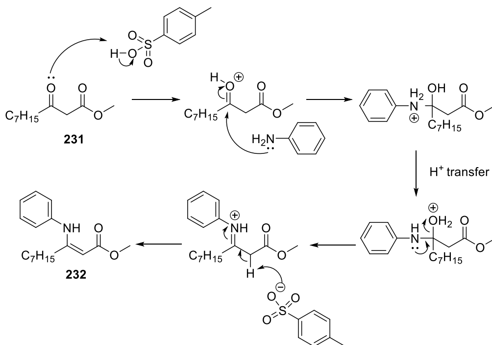
Scheme 5.3 Mechanism of formation of enamine from \beta -ketoester.
