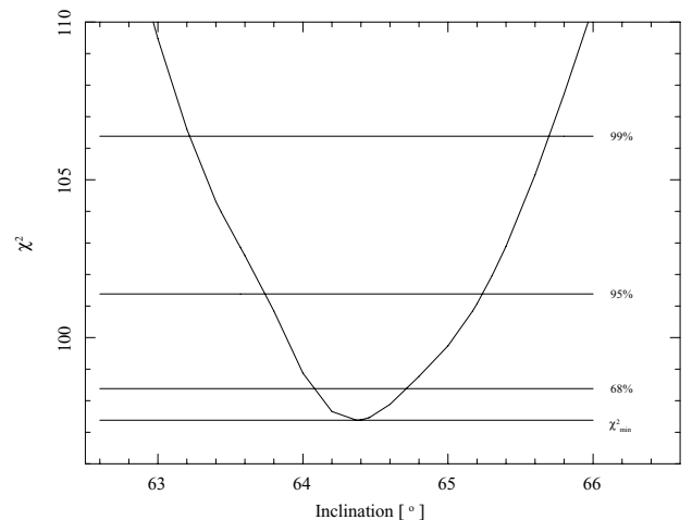
Figure 4. The graph of \chi^2 versus i for a pulsar of mass 1.4 M_{\odot} . Minimum occurs for \chi^2_{\nu} = 1.06 and an inclination, i \sim 64^{\circ}4 . The 68, 95 and 99 per cent confidence levels are illustrated.
