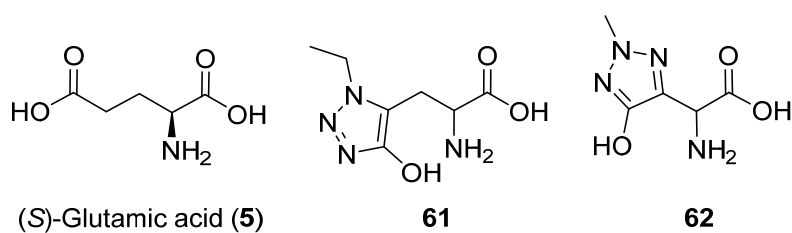
Figure 8 Structure of glutamic acid and its 4-hydroxy-1,2,3-triazole derivatives.
