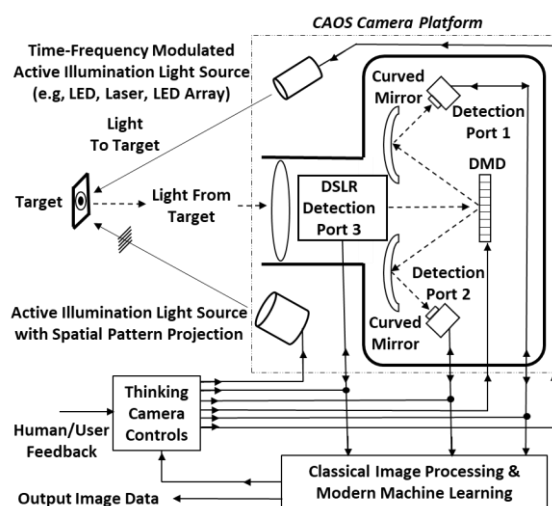
Figure 1 Thinking Camera Design empowered by the CAOS Camera Platform.
