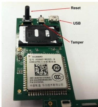
Figure 8(a). Image depicting the reset, USB and Tamper portions of the board. (b) Circuit diagram of the Tamper Switch.
