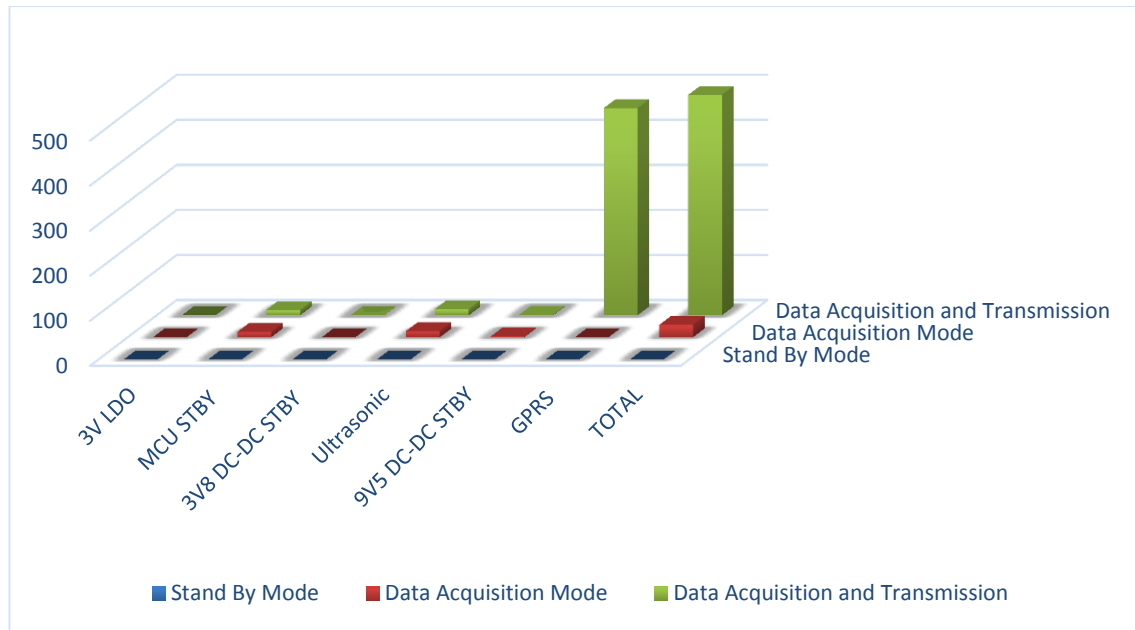
Figure 11. Graph of power Consumption.
