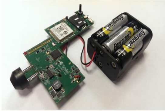
Figure 7(a). PCB Final Design
