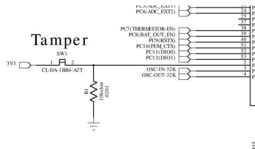
Figure 8(a). Image depicting the reset, USB and Tamper portions of the board. (b) Circuit diagram of the Tamper Switch.
