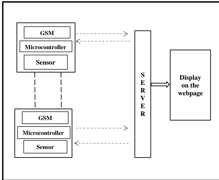
Figure 3. System Block Diagram.
