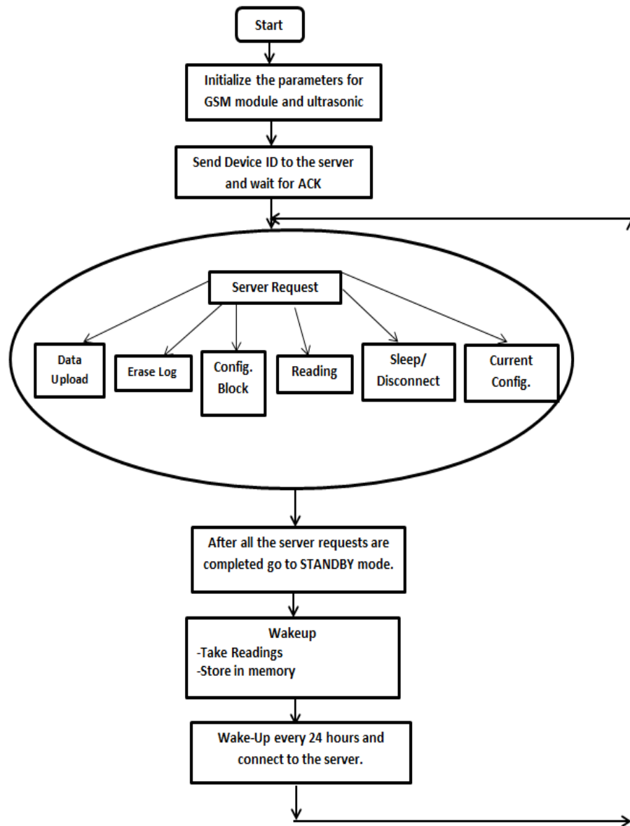
Figure 9. Flowchart.
