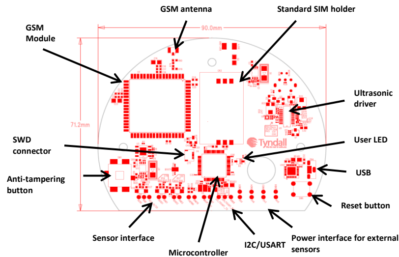
Figure 4. Placement of various components on the PCB (version 2)
