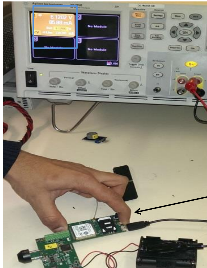
Figure 12. Power Testing Setup.
