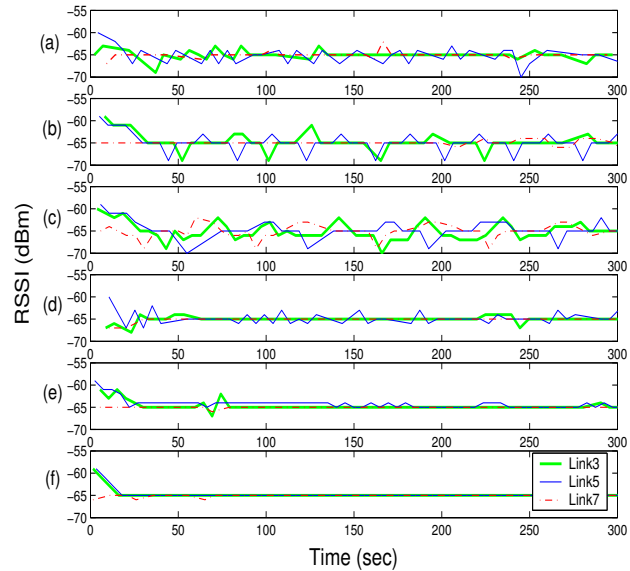
Fig. 9 Reference Node Power Control
