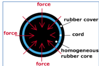
Fig. 9: Seaflex® component
