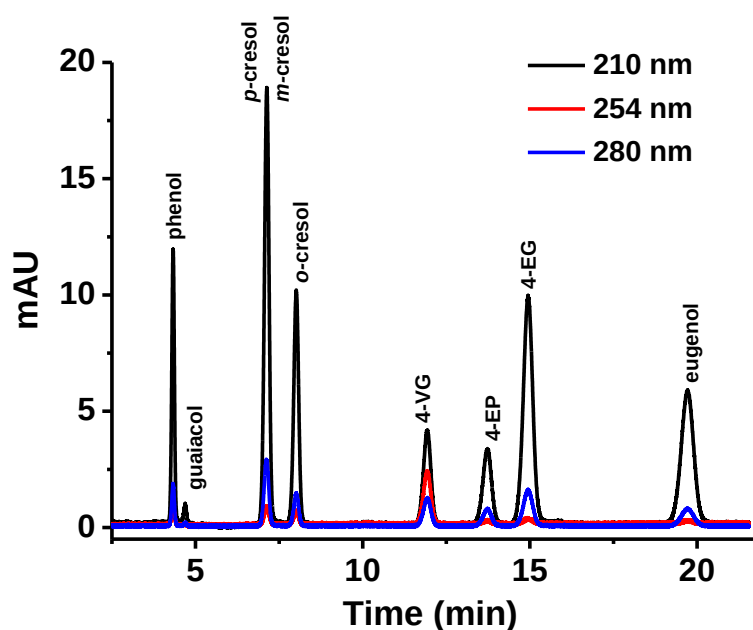
Figure 2.26. HPLC chromatograms of 40 \mu\text{M} of each standard at different wavelengths (210, 254, and 280 nm). Column: Agilent Eclipse XDB \text{C}_{18} (4.6 \times 150 mm, 5 \mu\text{m} ), mobile phase: 30: 70 ACN: \text{H}_2\text{O} (v/v, %), flow rate: 1 mL/min, injection volume: 5 \mu\text{L} , column temperature: 25 ^\circ\text{C} .
