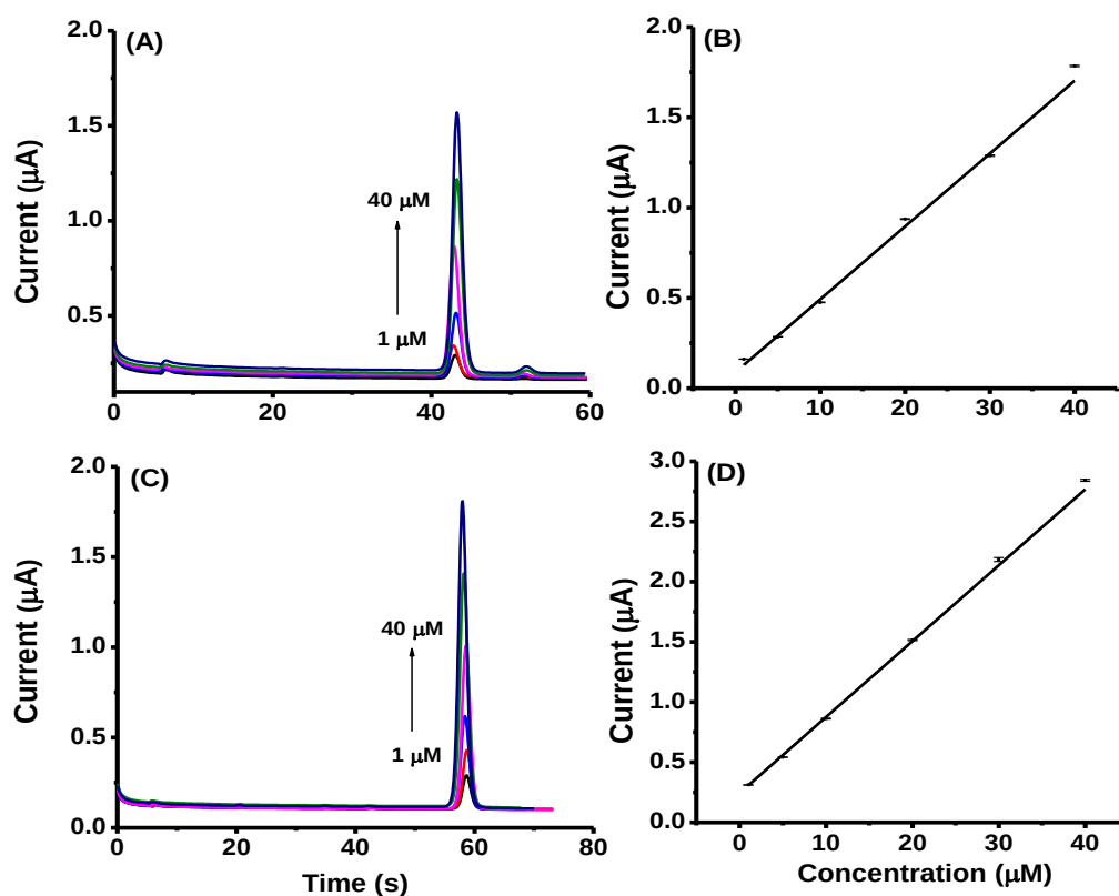
Figure 5.11. (A) Calibration curve and (B) plot of FA; (C) calibration curve and (D) plot of guaiacol. Mobile phase: ACN:10 mM formate pH 3, 17:83 (v/v). Column: HALO C_{18} core-shell (3 x 50 mm, 2.7 \mu m), flow rate: 1.3 mL/min, injection volume: 5 \mu L, oxidation potential: + 1.6 V on the BDD electrode vs. Pd/H 2 .
