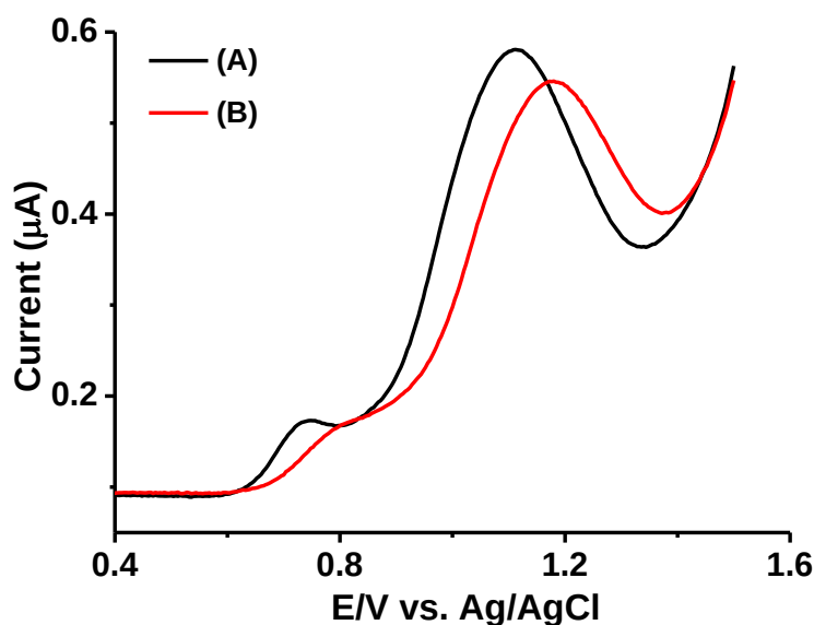
Figure 2.10. SWV of a standard mixture of phenol, guaiacol, o-cresol, m-cresol, p-cresol, 4-EP and 4-EG at 4 \mu M each, using 100 mM phosphate buffer, pH 2 with 5 % EtOH in the (A) absence and (B) presence of 10 mM \alpha -CD. Detection was achieved on the bare BDD electrode vs. Ag/AgCl.
