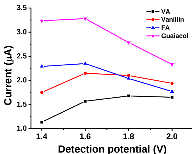
Figure 5.8. The plot of detection potential (V) versus current ( \mu\text{A} ) on the BDD electrode vs. Pd/H 2 . Mobile phase: ACN:10 mM formate pH 3 17:83, (v/v). Column: HALO C 18 core-shell (3 \times 50 mm, 2.7 \mu\text{m} ), flow rate: 1.3 mL/min, injection volume: 5 \mu\text{L} .
