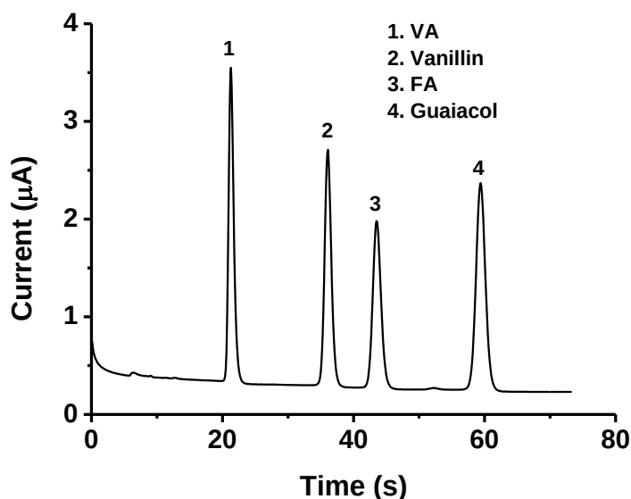
Figure 5.9. A representative HPLC-ECD chromatogram of a mixed standard solution (50 \mu\text{M} each of VA, vanillin, FA, and guaiacol). Mobile phase: ACN:10 mM formate pH 3, 17:83 (v/v). Column: HALO \text{C}_{18} core-shell (3.0 \times 50 mm, 2.7 \mu\text{m} ), flow rate: 1.3 mL/min, injection volume: 5 \mu\text{L} , oxidation potential: + 1.6 V on the BDD electrode vs. \text{Pd}/\text{H}_2 .
