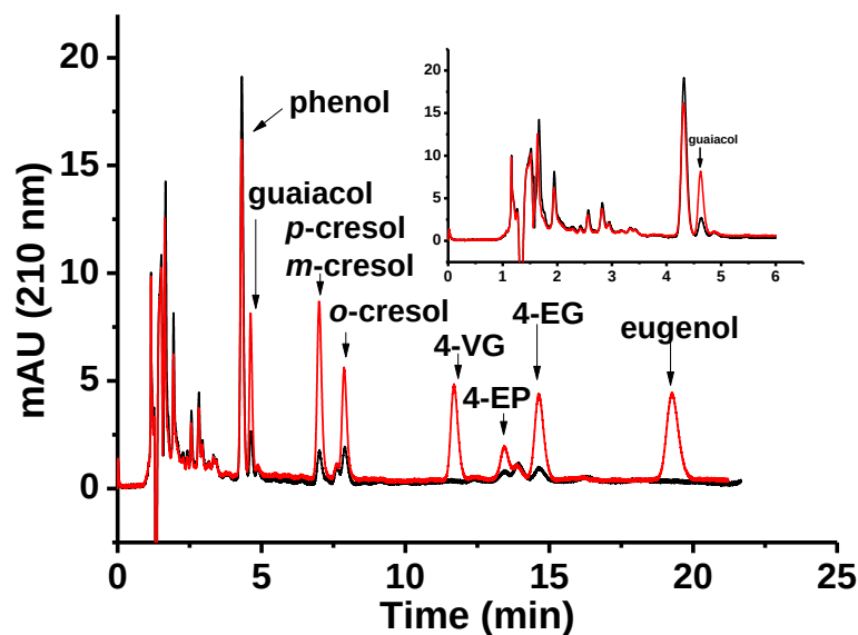
Figure 2.25. HPLC chromatograms of the 10-year-old blank Islay whiskey (black line) and spiked whiskey (red line) with 20 \mu\text{M} of each standard. Column: Agilent Eclipse XDB \text{C}_{18} (4.6 \times 150 mm, 5 \mu\text{m} ), mobile phase: 30: 70 ACN: \text{H}_2\text{O} (v/v, %), flow rate: 1 mL/min, injection volume: 5 \mu\text{L} , column temperature: 25 ^\circ\text{C} , UV detection: 210 nm.
