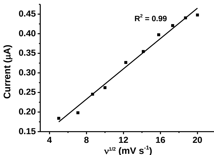
Figure 4.2. A plot of peak current versus square root of the scan rate ( v^{1/2} (mV s -1 )) for 100 \mu M GA at pH 2 on the BDD electrode vs. Ag/AgCl. The supporting electrolyte was 100 mM phosphate buffer with 5 % EtOH.
