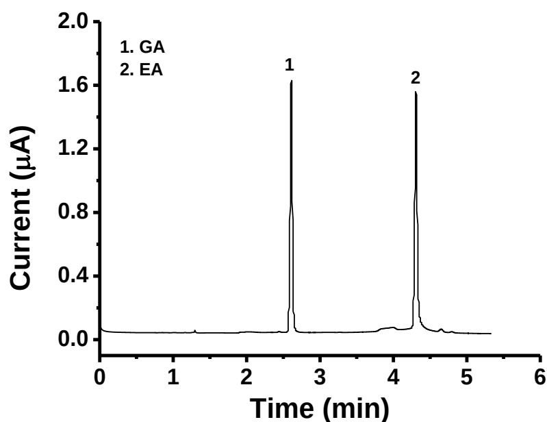
Figure 4.10. A 50 \mu\text{M} standard mixture of GA and EA. Column: Agilent XDB C_{18} (4.6 \times 150 mm, 5 \mu\text{m} ), mobile phase flow rate: 1.5 mL/min, injection volume: 5 \mu\text{L} , oxidation potential: + 1.4 V on the BDD electrode vs. Pd/H 2 .
