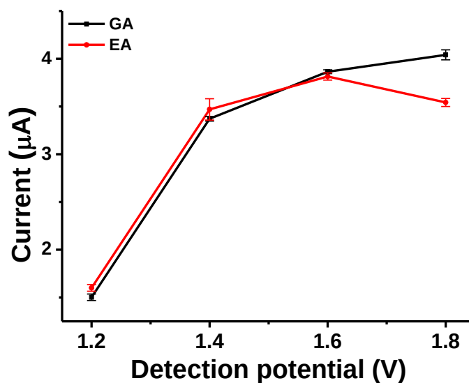
Figure 4.12. The plot of detection potential (V) versus current ( \mu\text{A} ) on the BDD electrode vs. \text{Pd}/\text{H}_2 . Column: Agilent XDB \text{C}_{18} (4.6 \times 150 mm, 5 \mu\text{m} ), mobile phase flow rate: 1.5 mL/min, injection volume: 5 \mu\text{L} .
