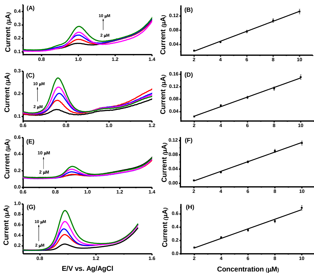
Figure 2.14. (A) Calibration curve and (B) plot of phenol; (C) calibration curve and (D) plot of guaiacol; (E) calibration curve and (F) plot of o-cresol and (G) calibration curve and (H) plot of m-cresol. The electrolyte was 100 mM phosphate, pH 2 with 5 % EtOH containing 10 mM \alpha -CD. Detection was achieved on the Nafion modified BDD electrode vs. Ag/AgCl. Error bars represent the standard deviation.
