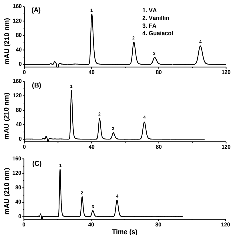
Figure 5.6. The effect of the mobile phase flow rate on the retention time of 50 \mu M each of VA, vanillin, FA and guaiacol. Mobile phase: ACN:10 mM formate pH 3, 17:83 (v/v). Column: HALO C_{18} core-shell (3.0 x 50 mm, 2.7 \mu m), flow rate: (A) 0.7 mL/min, (B) 1 mL/min, (C) 1.3 mL/min, injection volume: 5 \mu L, UV detection: 210 nm.
