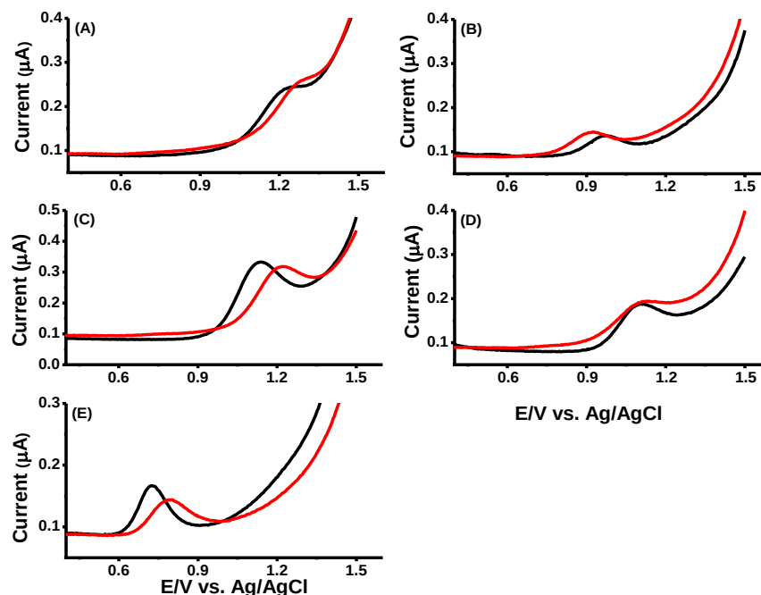
Figure 2.9. SWV of 4 \mu M (A) phenol, (B) guaiacol, (C) m-cresol, (D) 4-EP and (E) 4-EG, using 100 mM phosphate buffer, pH 2 with 5 % EtOH in the absence (black lines) and presence (red lines) of 10 mM \alpha -CD. Detection was achieved on the bare BDD electrode vs. Ag/AgCl.
