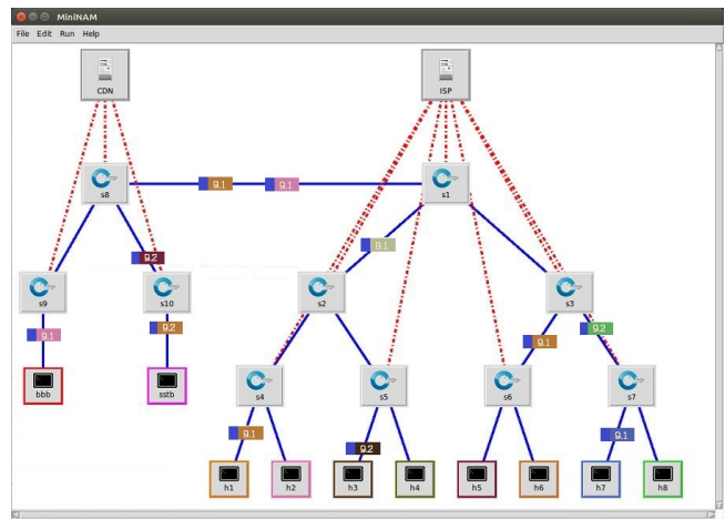
Fig. 4. A snapshot of MiniNAM with Tree topology
