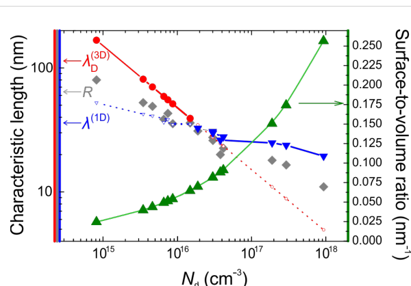
Figure 4: Characteristic length scales in Ge NWs. 3D Debye \lambda_D^{(3D)} and 1D screening length \lambda^{(1D)} as function of carrier density N_d . NW radius sizes (grey symbols) are plotted as a reference. Green triangles show the corresponding surface-to-volume ratios.
