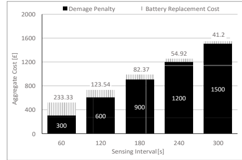
Fig. 8. Aggregate cost summarizing damage penalty and battery replacement cost when C_u = £10 , R_p = 30/\text{min}
