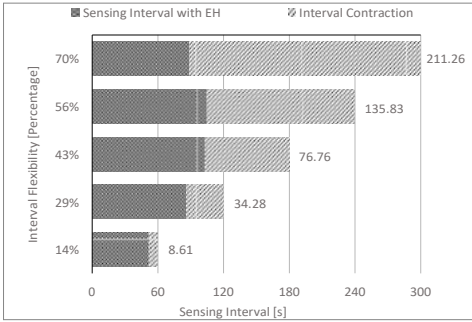
Fig. 11. Sensing interval flexibility and the rate of interval contraction when exploiting energy harvesting sources in industrial environment
