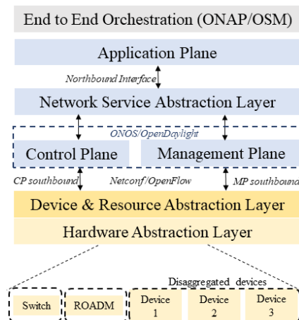
Figure 1. System Architecture within SDN framework defined in [1]
