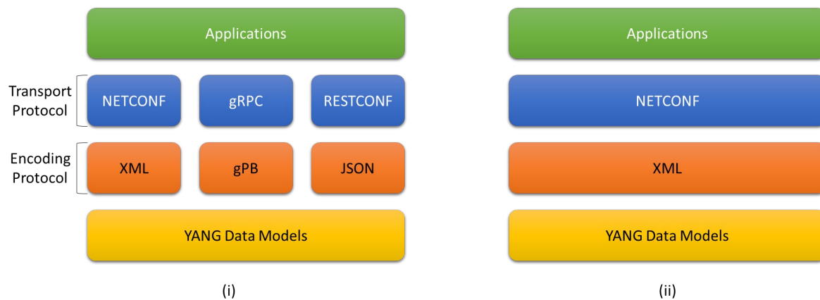
Figure 2. (i) Architecture choices for transport and encoding; (ii) One Implementation.
