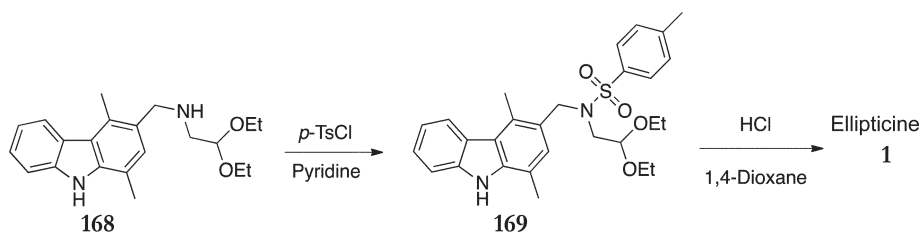
Scheme 34
