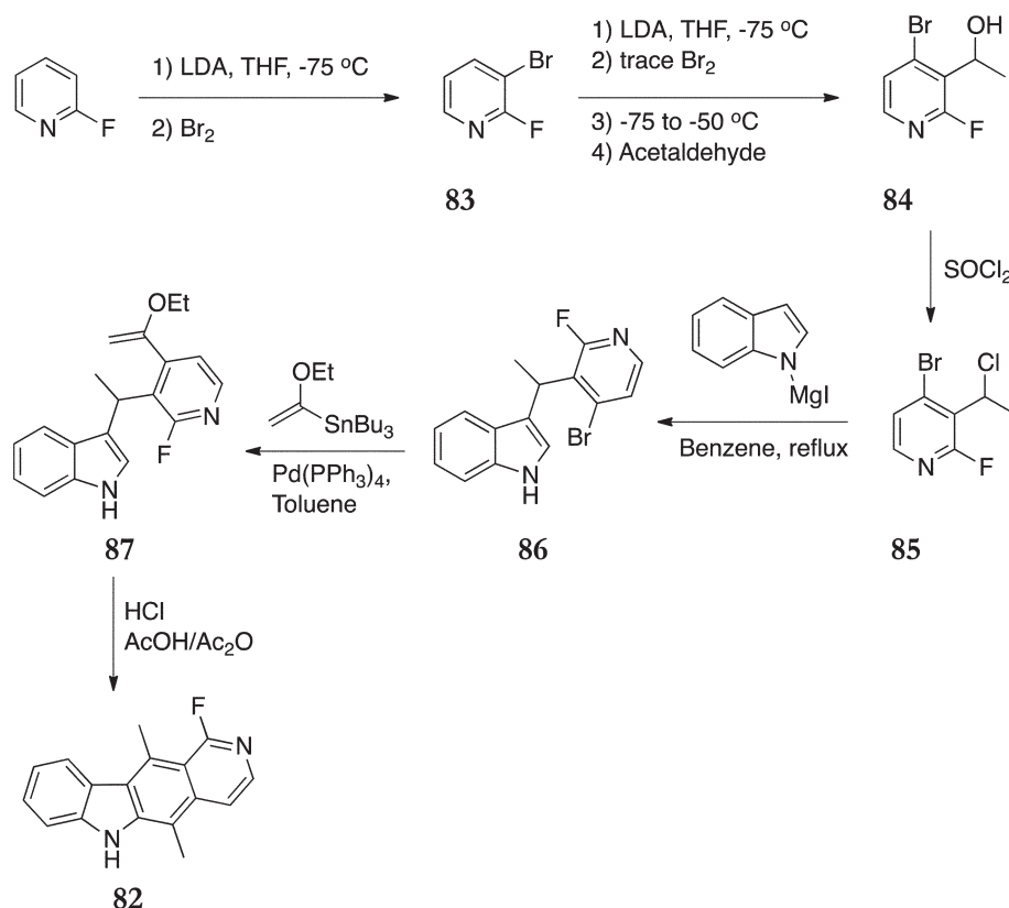
Scheme 17
