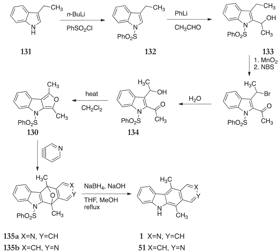
Scheme 25
