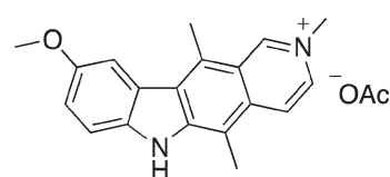
Fig. 5 9-Methoxy- N -methylellipticinium acetate 14 .
