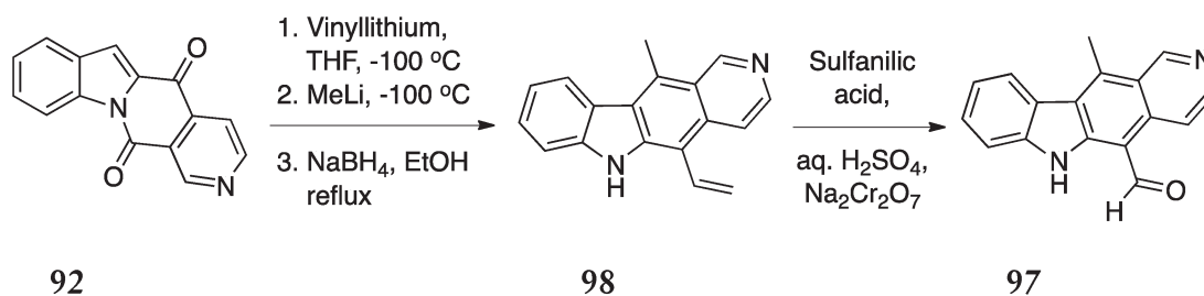
Scheme 19
