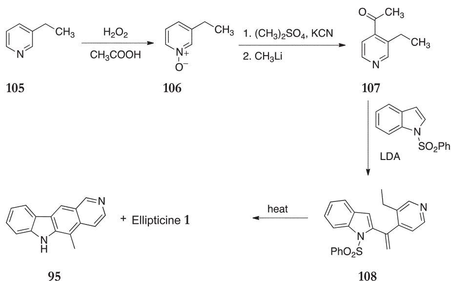
Scheme 21
