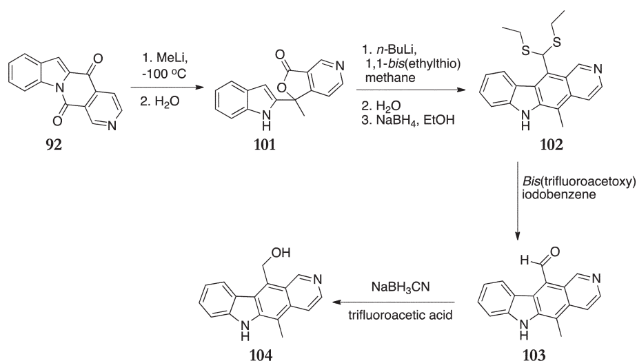
Scheme 20
