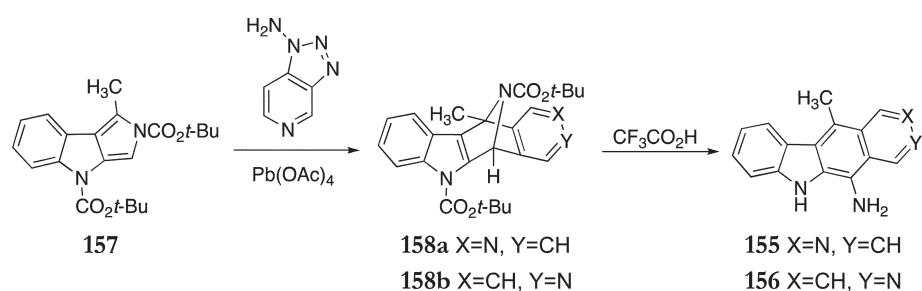
Scheme 29
