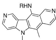
Fig. 13 9-Azaellipticine analogues 116.
