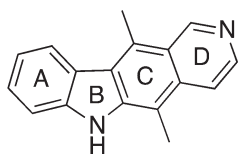
Fig. 1 Ellipticine 1.
