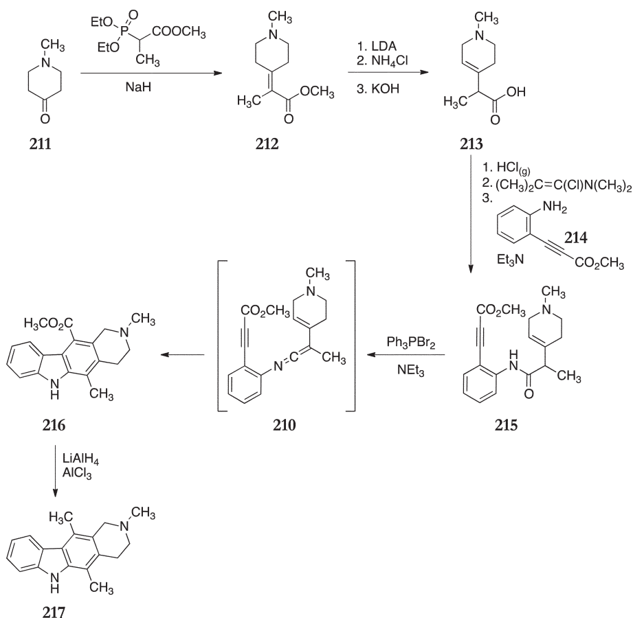
Scheme 48
