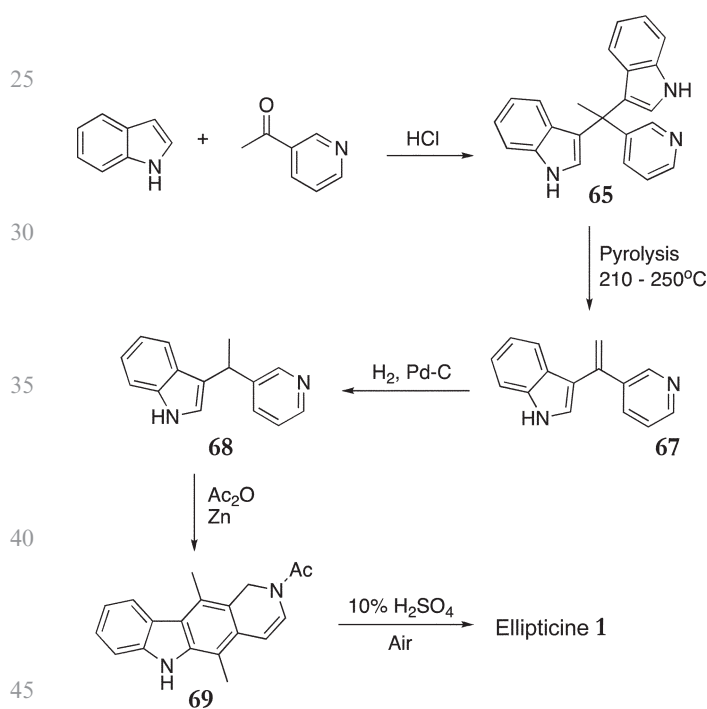
Scheme 14
