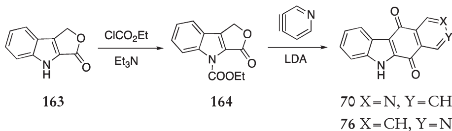
Scheme 32
