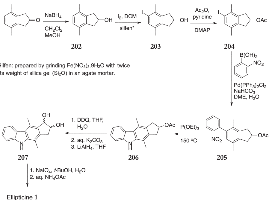
Scheme 46
