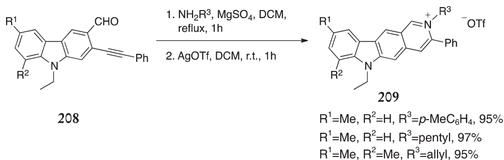
Scheme 47
