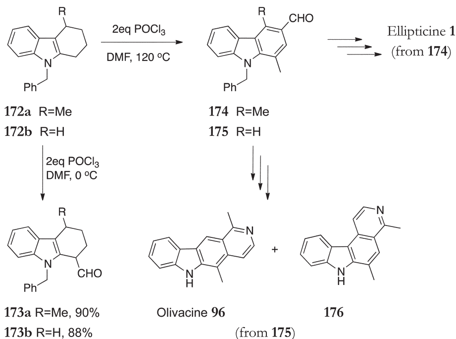
Scheme 36
