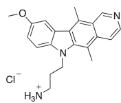
Fig. 6 3-(9-Methoxy-5,11-dimethyl-6H-pyrido[4,3-b]carbazol-6-yl)propan-1-aminium chloride 15 .
