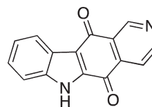
Fig. 9 Ellipticine quinone 70.
