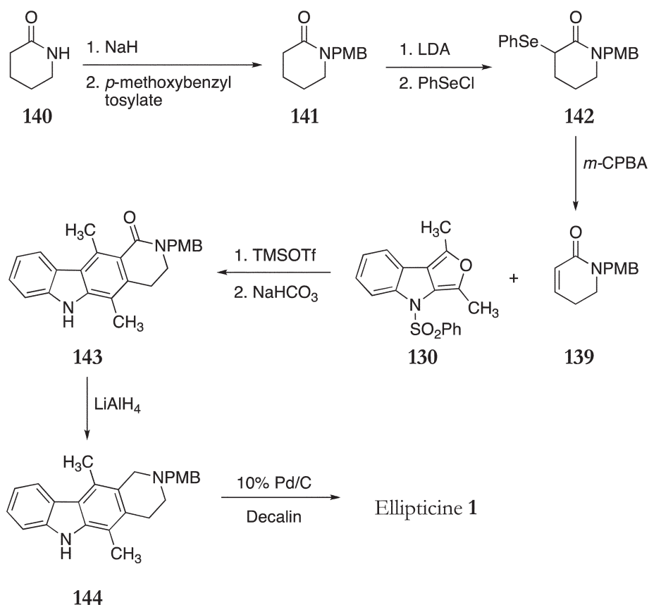
Scheme 27
