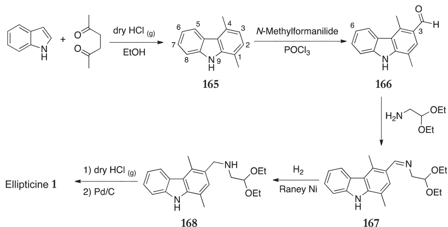
Scheme 33
