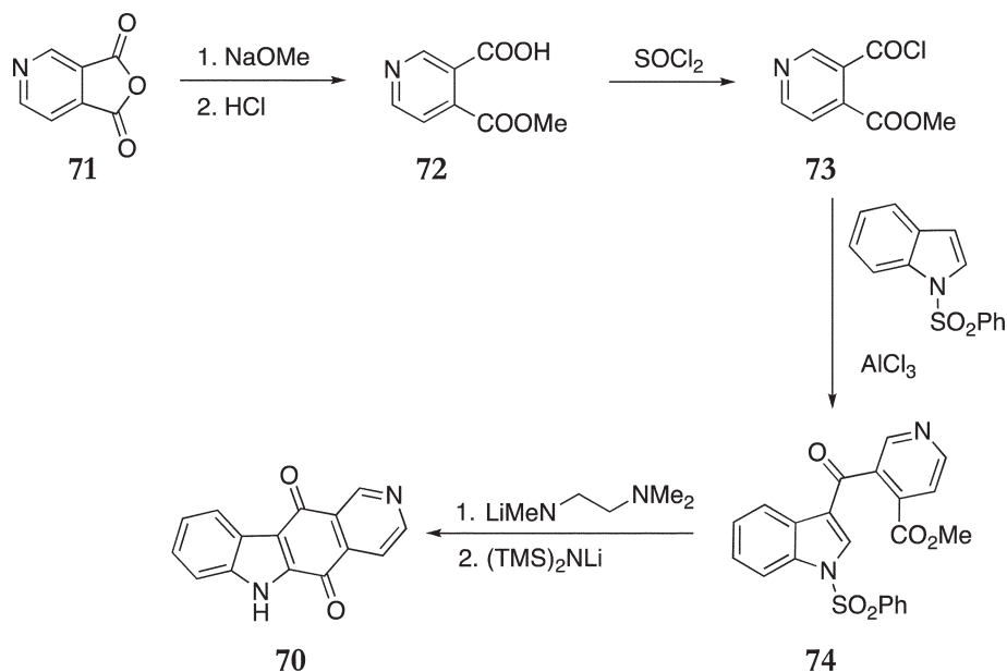
Scheme 15
