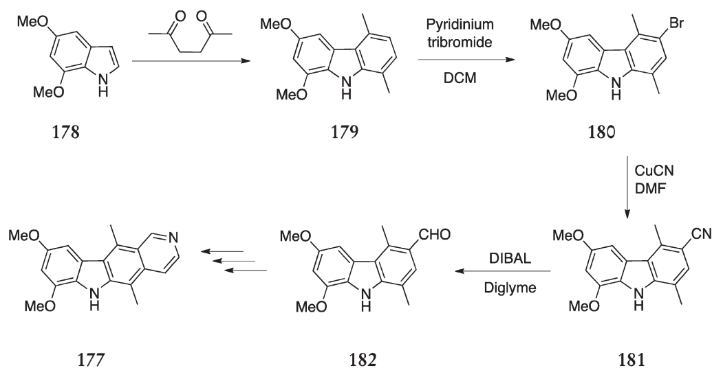
Scheme 37
