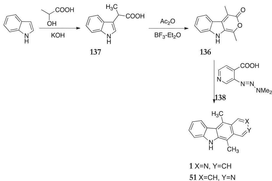
Scheme 26
