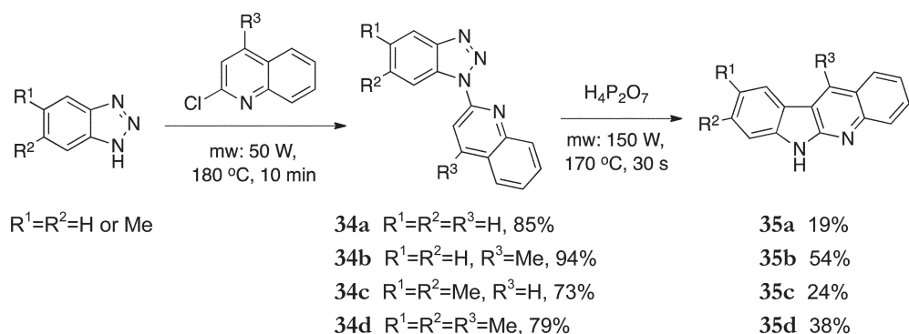
Scheme 7
