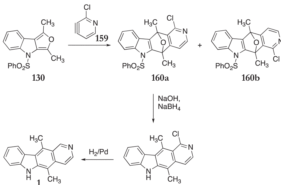
Scheme 30
