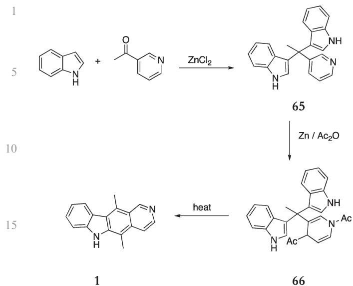
Scheme 13
