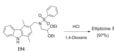
Scheme 41
