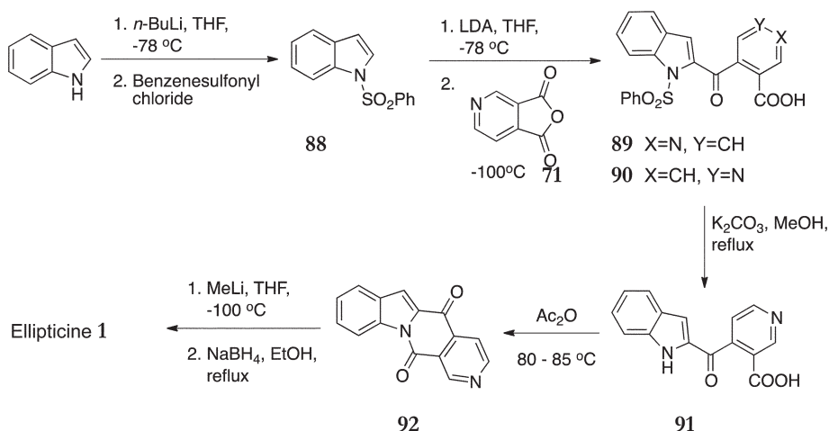
Scheme 18
