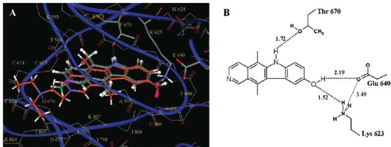
Fig. 3 (A) Detail of the docked position of the most active compounds (9-hydroxyellipticine 4 is shown in gray, 9-hydroxy- N -methylellipticinium 3 in green, and N -alkylamino-9-hydroxyellipticinium 10 in orange). Conserved interactions are represented by dashed lines. (B) Map of the main interactions for 9-hydroxyellipticine 4 . 27
