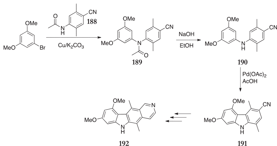
Scheme 39
