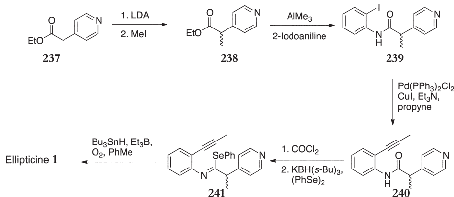
Scheme 51
