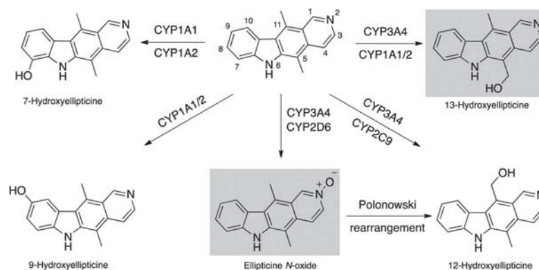
Scheme 2 Ellipticine metabolites formed by human cytochrome P450 enzymes. 18
