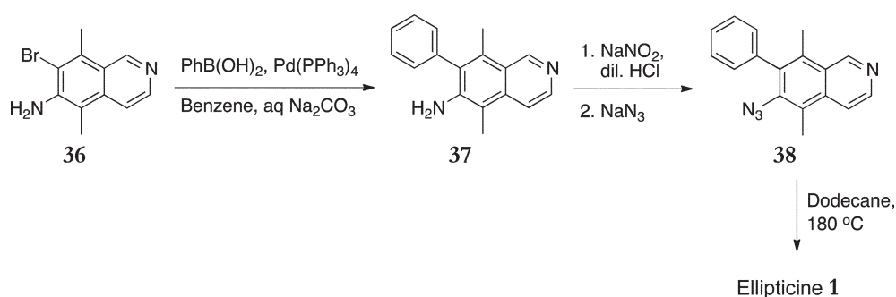
Scheme 8
