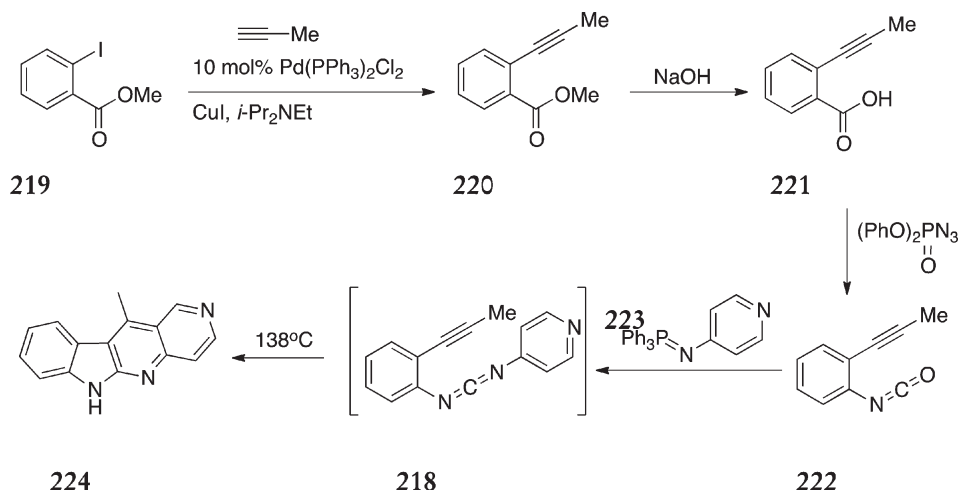
Scheme 49
