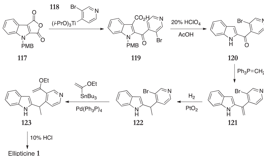
Scheme 23
