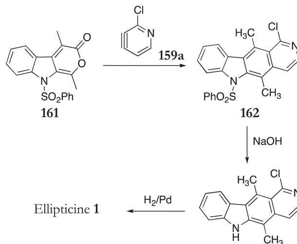
Scheme 31
