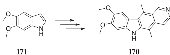
Scheme 35
