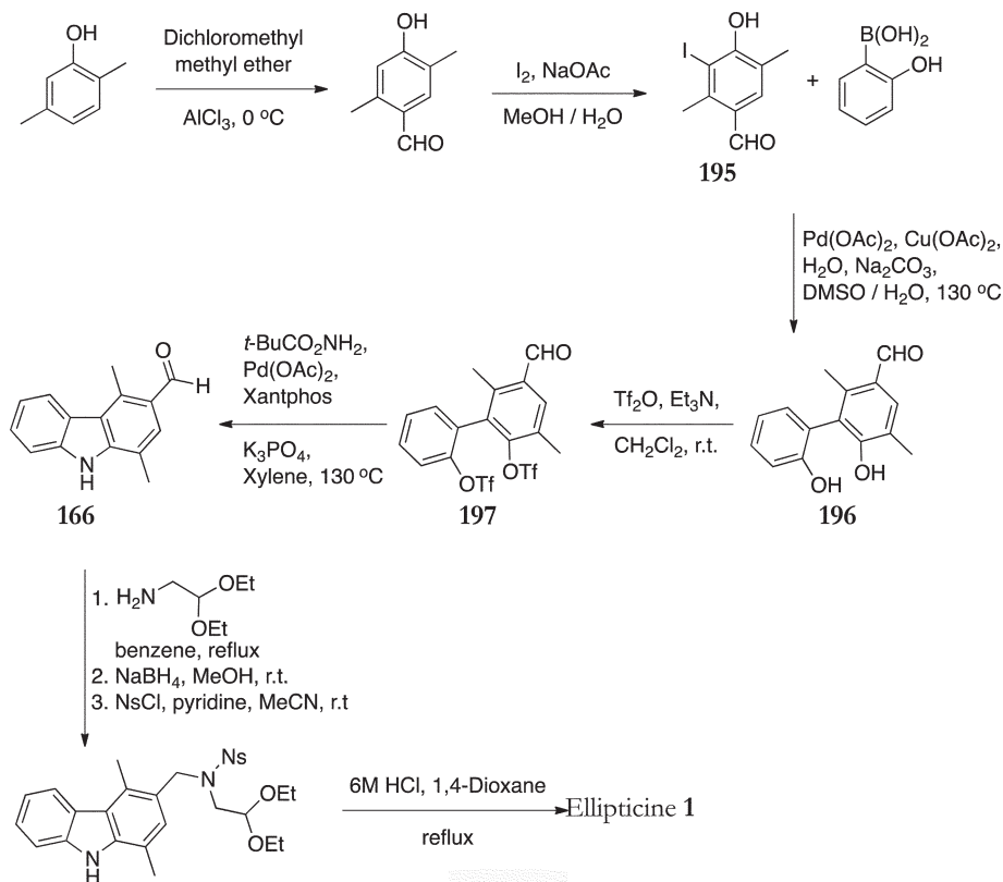
Scheme 43
