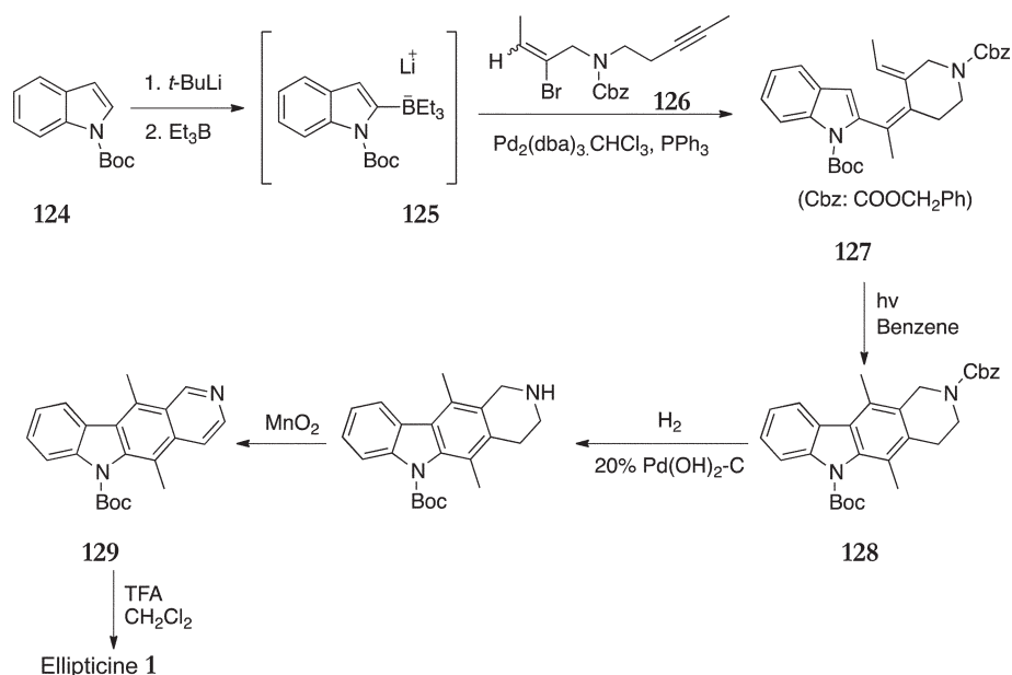
Scheme 24
