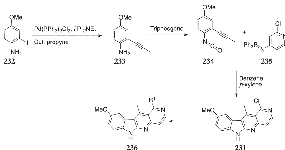
Scheme 50
