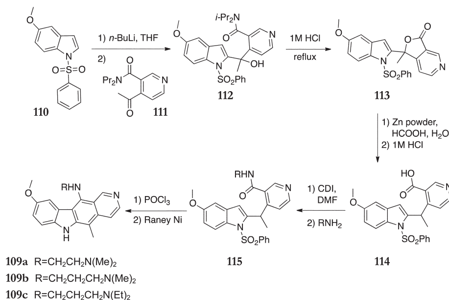
Scheme 22
