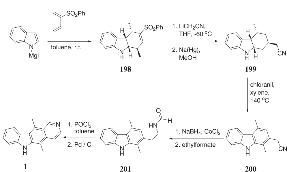
Scheme 45
