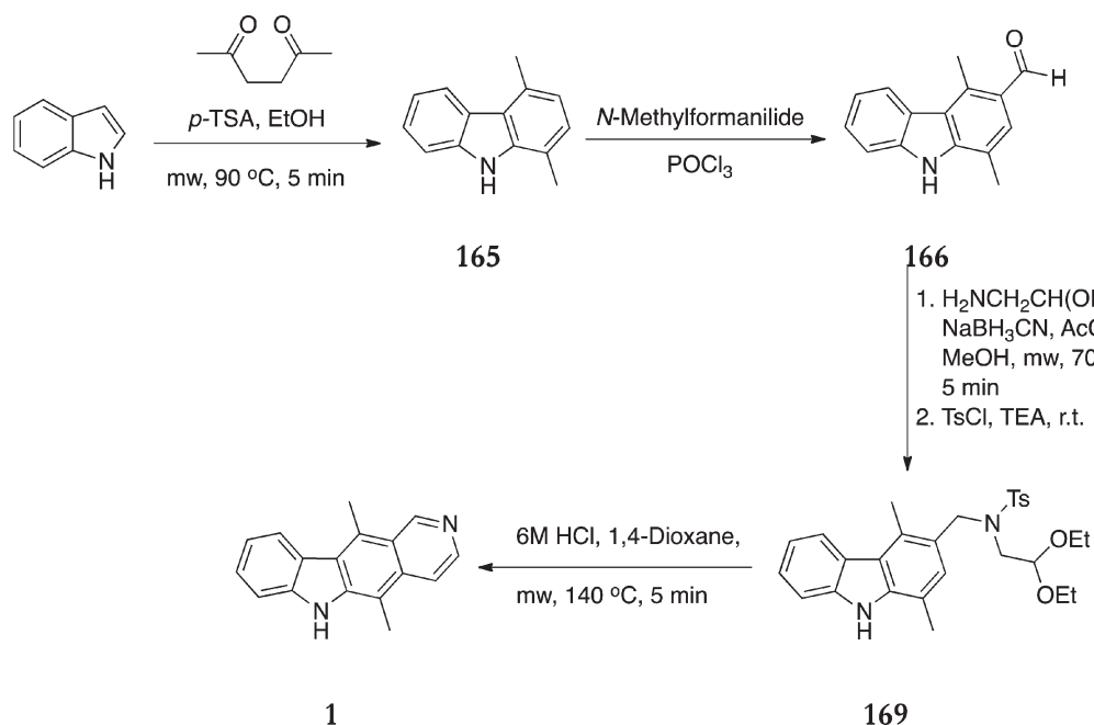
Scheme 42
