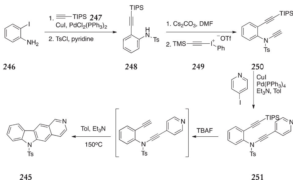
Scheme 53
