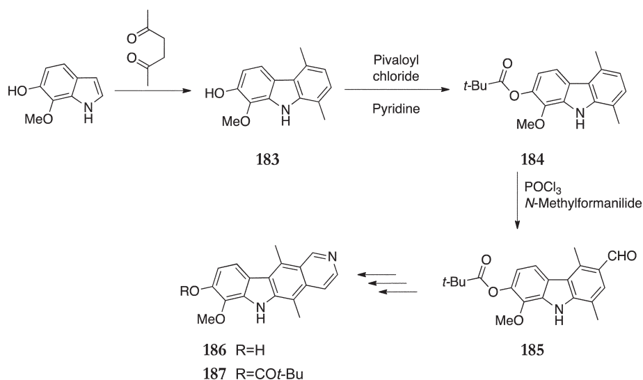
Scheme 38
