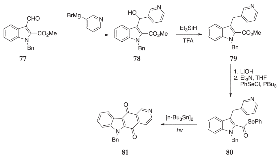
Scheme 16
