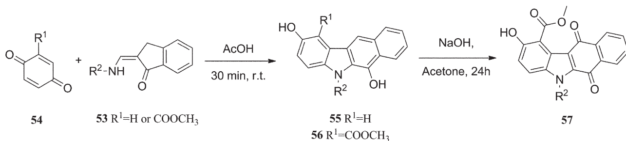
Scheme 11
