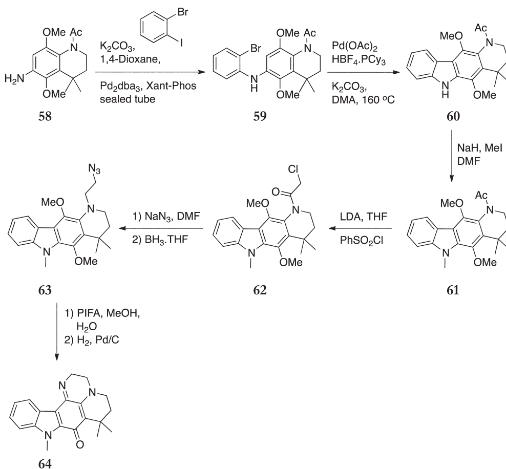
Scheme 12
