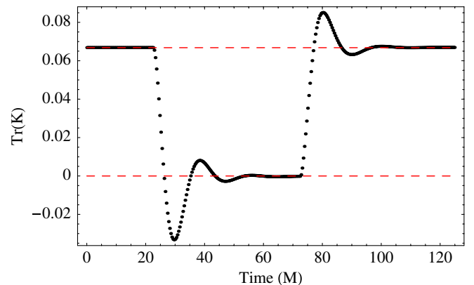
FIG. 21 (color online). The value of K at the horizon, for a simulation where the slicing condition alternates between standard 1 + log and asymptotically maximal 1 + log, Eqs. (21) and (36). The dashed horizontal lines indicate the respective analytic values of K at the horizon.
