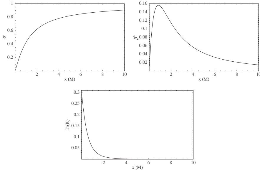
FIG. 5. The lapse \alpha , x -component of the shift vector \beta^x , and K for time-independent 1 + log data in isotropic coordinates. The data are shown along the x axis.
