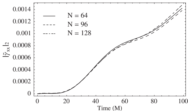
FIG. 20. The L_2 norm of the error in \tilde{\gamma}_{xx} over the course of the evolution. The errors again converge to zero at fourth order.
