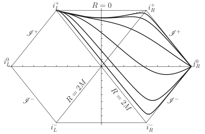
FIG. 4. The Penrose diagram of the slices defined by the stationary solution of the 1 + \log condition with n = 2 . Every slice approaches i_L^+ along the curve R = R_0 \approx 1.31M and spatial infinity i_R^0 along a curve of constant T . The slices are displayed in time steps of 4M .
