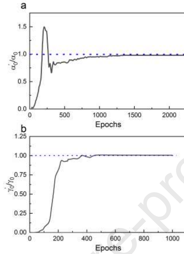
Figure 10 Kernel parameter estimations by PBNN (a) aggregation rate constant estimation (b) breakage rate constant estimation
