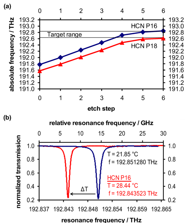
FIG. 3. (a) Simultaneous tuning of two different microresonators located on the same chip. The graphs show the reproducibility of the different etching steps and between consecutive steps with same processing time. The first 4 steps each had a duration of 60 s, the following steps had reduced etching times of 30 s and 6 s. (b) After approaching a specific resonance line (HCN P16), final tuning within a few GHz was done by simple thermal shifting with the Peltier element from our temperature control setup.
