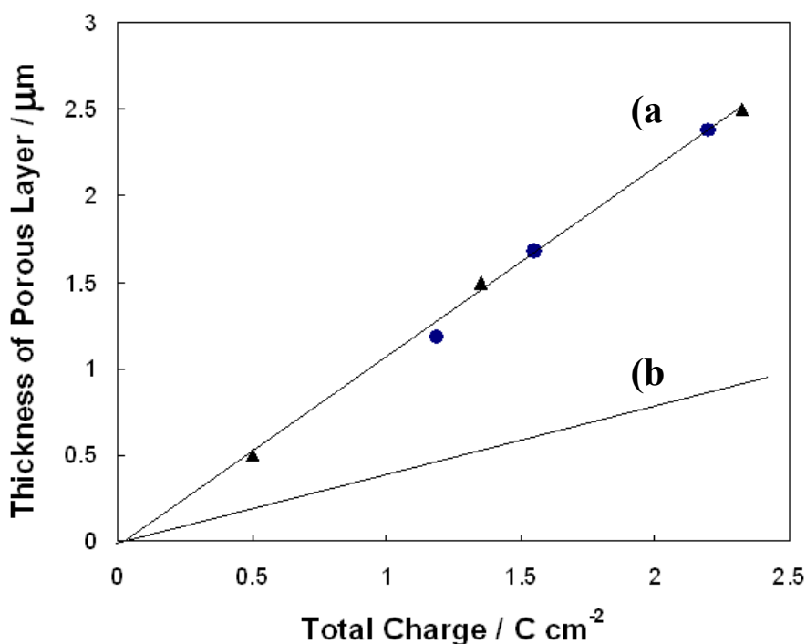
Fig. 8 Plot of porous layer thickness for samples anodized at constant potential (●) and after potential sweep (▲) as a function of the charge passed. (-) Theoretical thickness of InP removed.
