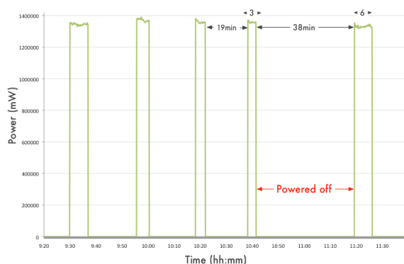
Figure 6. Illustration of the time taken by the heater to reach its optimum temperature after various off durations
