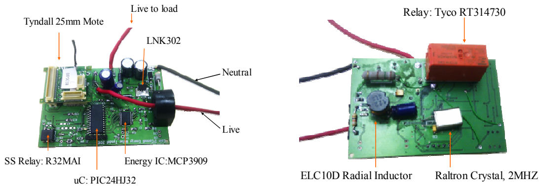
Figure 1. Labeled REAM plug layer top and bottom
