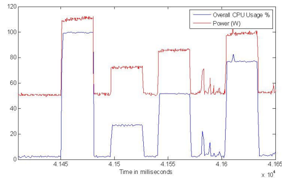
Figure 3. Power profile of HP Compaq dc9700
