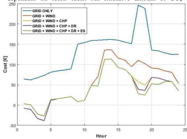
Fig. 4. Cost profile for 14th February 2017.
