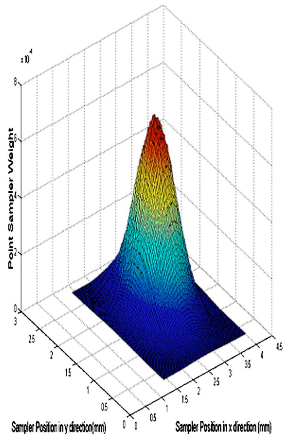
FIG. 4. (Color online) Plot showing computed VOA control weights in 2D for the spatial samplers in the DMD™. Plot is generated using experimental data shown in Figs. 2 and 3.
