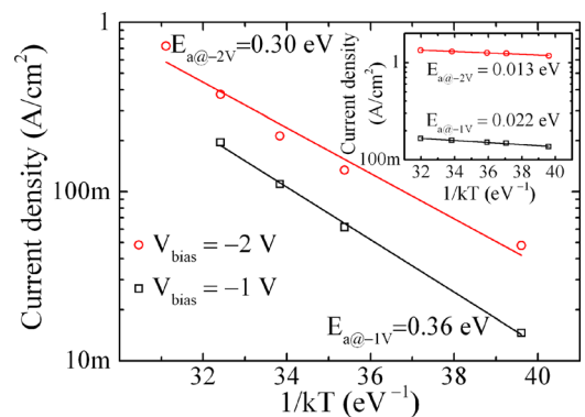
FIG. 3. (Color online) Current density versus 1/kT at 1\ \text{V} and 2\ \text{V} reverse bias voltages before annealing. The circular and square symbols are the measured data and the solid lines are the Arrhenius-fit plots. The inset shows the same plot after annealing. The value of the activation energy at each bias voltage is also shown.
