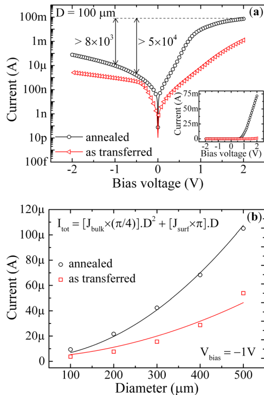
FIG. 2. (Color online) (a) I - V characteristic of a 100\ \mu\text{m} -diameter diode before and after annealing. The ideality factor of the diode is 5.48 before annealing and 2.28 after annealing. The inset shows the I - V characteristic in linear scale. (b) Current versus device diameter at 1\ \text{V} reverse bias before and after annealing; circular and square symbols: measured data; solid lines: fit from bulk leakage (per unit area) and surface leakage (per unit diameter).
