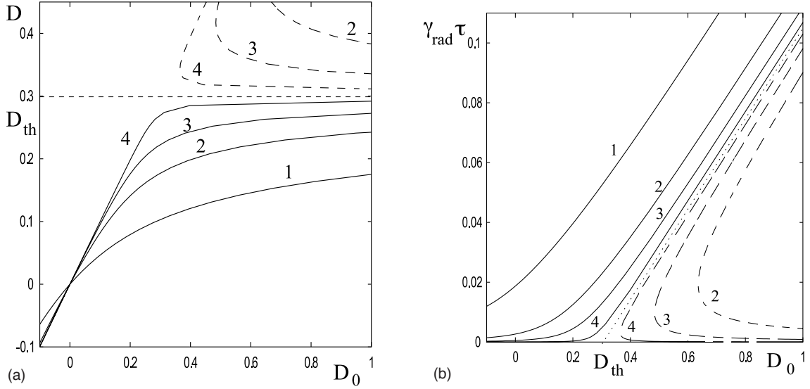
FIG. 2. (a) Normalized gain (population inversion D ) of the two-level system in the DNL and (b) DNL radiation rate versus the normalized pump rate for various intensities of external field taken in units of saturated intensity for the two-level system, with I=0.7 (curves 1), 0.1 (2), 0.02 (3), 0.001 (4). The dashed curves correspond to unstable stationary solutions with D > D_{th} .
