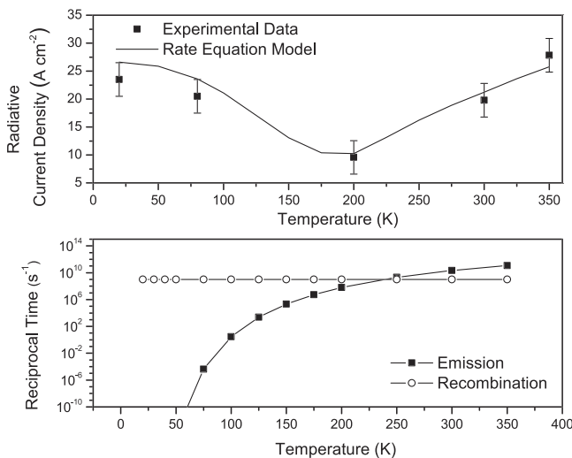
FIG. 1. Upper diagram shows the temperature dependence of radiative threshold current of a quantum dot laser emitting at 1.3\ \mu\text{m} (points) and a rate equation calculation (line). Reproduced with permission from I. O'Driscoll, P. Blood, and P. M. Smowton, IEEE J. Quantum Electron. 46 (4), 525 (2010). Copyright 2010 IEEE Photonics Society. The lower diagram shows the reciprocals of the component ground state phonon-induced emission (solid squares) and radiative recombination times in a dot (open circles), the latter from measured absorption spectra via the Einstein relations.
