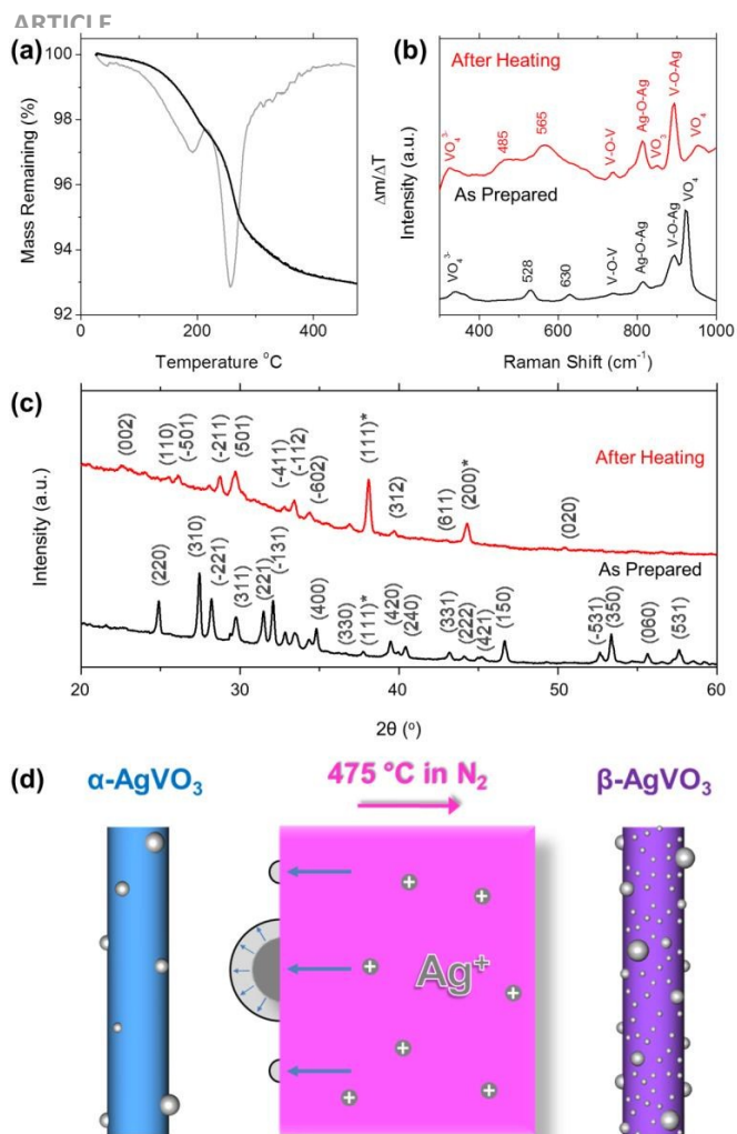
Fig. 2. (a) Thermogravimetric analysis and derivative mass loss curves for AgVO 3 nanowires heated to 475 °C in N 2 at a ramp rate of 5 °C/min (b) Raman spectra and (c) XRD patterns of AgVO 3 nanowires before and after heating to 475 °C in N 2 . Reflections labelled with * correspond to cubic Ag. (d) Schematic representation of the transition from α-AgVO 3 to β-AgVO 3 upon heating to 475 °C in N 2 .
