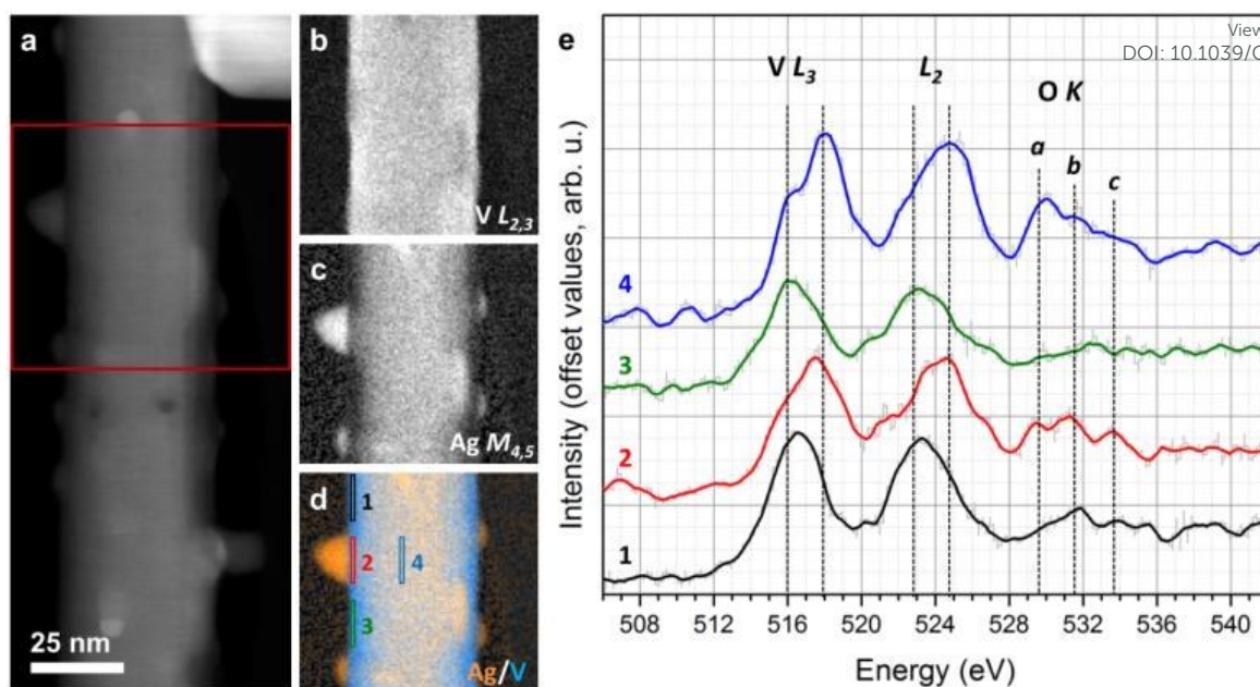
Fig. 4. (a) HAADF image of a typical \beta -AgVO 3 nanowire, EELS maps showing contributions from (b) V L and (c) Ag M edges, (d) an overlay of V L and Ag M edge maps demonstrating the distribution of V and Ag in the \beta -AgVO 3 NWs, (e) EELS spectra acquired from the four areas of the \beta -AgVO 3 NW highlighted in (d).
