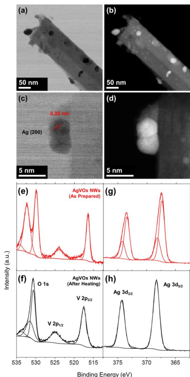
Fig. 3. Bright field (a) and dark field (b) STEM images of an Ag NP-decorated \beta -AgVO 3 NW. Bright field (c) and dark field (d) STEM images of an Ag NP. XPS spectra of O 1s and V 2p regions for AgVO x NWs (e) before and (f) after heating to 475 °C in N 2 . XPS spectra of the Ag 3d region for AgVO x NWs (g) before and (h) after heating to 475 °C in N 2 .
