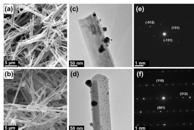
Fig. 1. SEM images (a) and (b), TEM images (c) and (d) and electron diffraction patterns (e) and (f) of AgVO x nanowires before and after heating to 475 °C in N 2 .
