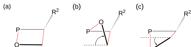
Fig. 8. (a) Planar TS with pucker angle of 0°, (b) TS with positive pucker angle, (c) TS with negative pucker angle.
