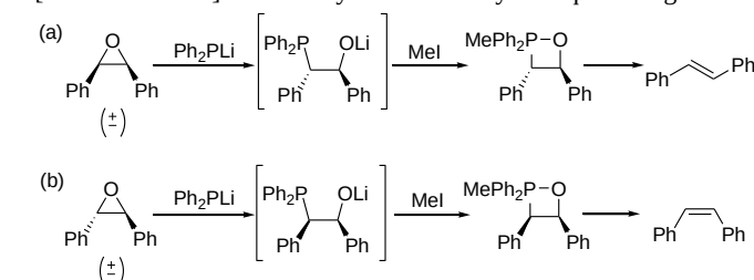
Scheme 17. Stereospecific conversion of (a) cis -stilbene oxide to E -stilbene and (b) trans -stilbene oxide to Z -stilbene by nucleophilic ring cleavage and quaternisation of the resulting \beta -oxidophosphine.
