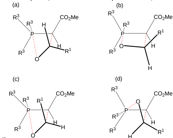
Fig. 11. (a) Favoured trans -selective TS showing negative puckering angle, (b) Lowest energy cis -selective TS, (c) & (d) Higher energy cis -selective TSs.
