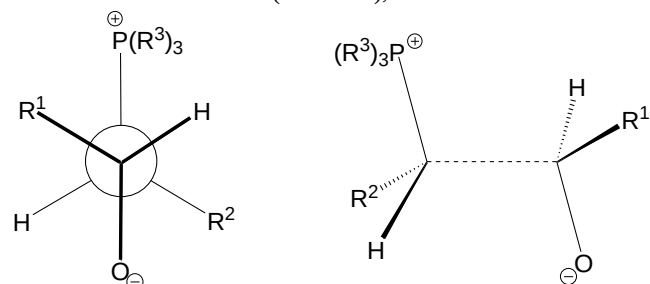
Fig. 2. Two diagrams of the transition state leading to the anti -conformer of erythro -betaine, which has been proposed as the kinetically favoured path for the Wittig reaction.
