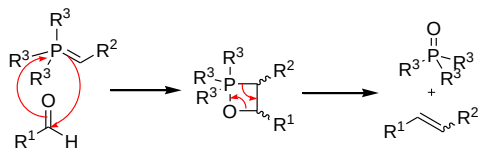
Scheme 13. The irreversible [2+2] cycloaddition mechanism of Vedejs.
