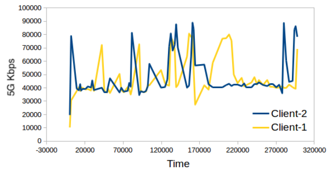
Fig. 1. Throughput variation of two clients streaming over 5G
