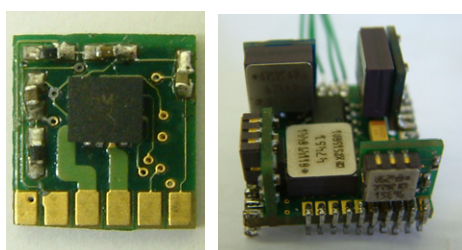
Figure 4. IMU board Designs and interconnect technique.
