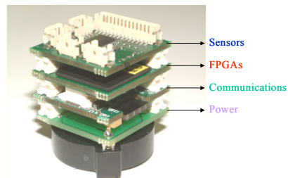
Figure 2. 25mm Platform.
