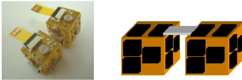
Figure 5. Assembled Flex cubes and Berries concept
