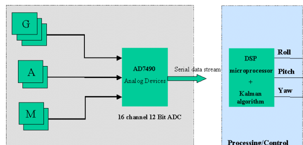
Figure 3. IMU Architecture
