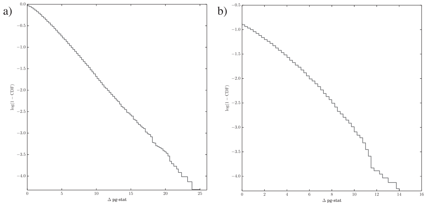
Figure 6. Complementary cumulative distribution function of the pg-stat obtained for models (a) f_{\text{BHec}} function vs. BB + f_{\text{BHec}} , and (b) BB + Band function vs. BB + f_{\text{BHec}} are shown.
