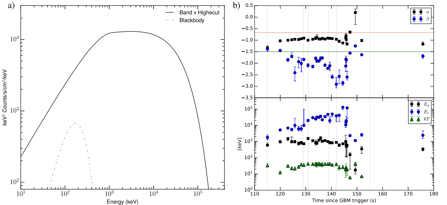
Figure 4. Panel (a): the \nu F_\nu plot of the best-fit model, Band \times Higecut (solid black line) + blackbody (BB; dashed–dotted black line), fitted to the brightest time interval, i.e., 134.59–135.71 s. Panel (b): the upper section shows the time evolution of \alpha (black squares) and \beta (blue circles) of the Band function. The green and red horizontal lines in the upper section mark the photon index of \alpha = -1.5 and \alpha = -0.67 , corresponding to the fast and slow cooling synchrotron emissions, respectively. In the lower section, the time evolution of the Band E_p (black squares), the high-energy cutoff E_c (blue circles), and the temperature of the BB component kT (green triangles) are shown. The three time intervals of polarization study are shown in dotted vertical black lines across the two panels.
