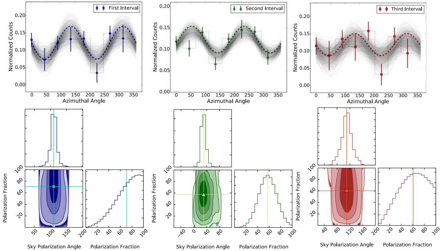
Figure 2. Top-left corner: for the first interval, the best-fit modulation curve obtained is shown in dashed blue line. Modulation fits obtained for 1000 out of \sim 10^7 simulated data sets are shown here in shaded black. In the bottom-left corner, the 2D histogram plot of the obtained PF and PA values, along with the contours corresponding to confidence levels of 68%, 90%, 99%, and 99.9%, are shown in terms of darker to lighter shades of blue, which are overplotted on the scatter plot of PF and PA. Similar corresponding plots for interval 2 are shown in the top-middle and bottom-middle panels (green). For this time interval, an additional contour of confidence level 99.99% is shown in the 2D histogram plot. For interval 3, corresponding plots are shown in the top-right corner and bottom-right corner (red). The average values of PF and PA obtained in intervals 1, 2, and 3 are marked by the blue circle, green triangle, and red square, respectively, on their 2D histograms; they are also marked by solid lines on their respective posterior distribution plots.
