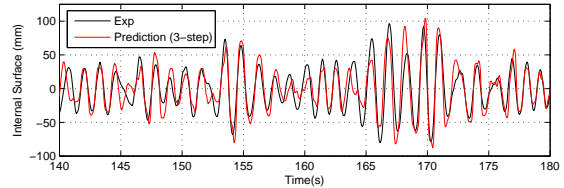
Figure 9 Short-term prediction of water height in column
