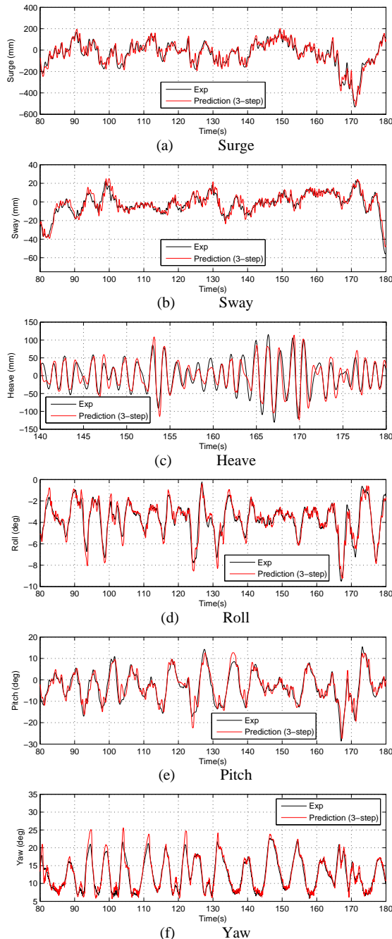
Figure 8 Short-term predictions of motions of the floating OWC
