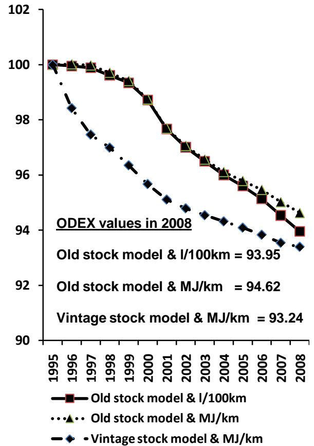
Figure 4 All calculated versions of the Irish private car ODEX
