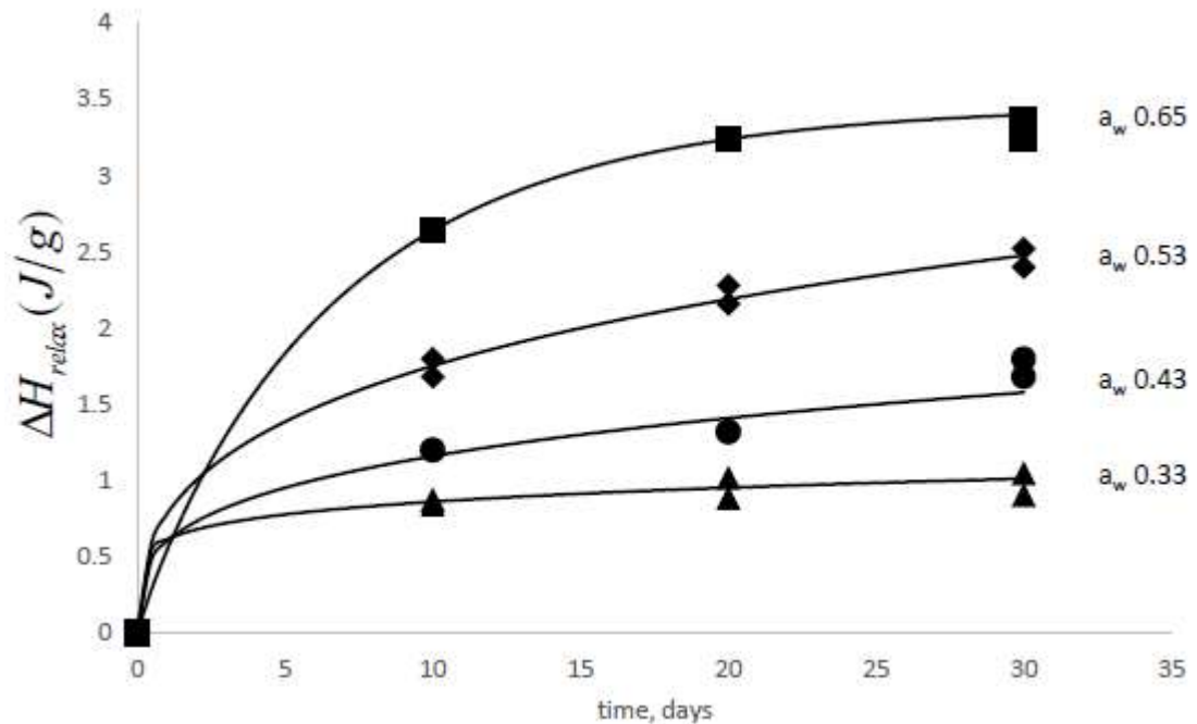
Fig.2.5. Enthalpy relaxation ( \Delta H_{relax} ) data and calculated enthalpy relaxation using KWW model against ageing time of Maltodextrin at various water activities.
