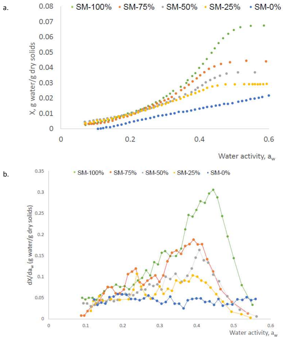
Fig.3.6. Comparison of sucrose-maltodextrin with different ratios of amorphous sucrose to crystalline sucrose (solid/solid, maltodextrin in fix ratio). Five amorphous/crystalline were made 100 %, 75 %, 50 %, 25 % and 0 %, namely, SM-100, SM-75%, SM-50%, SM-25% and SM-0%, respectively. (a) Dynamic water sorption of sucrose-maltodextrin systems. (b). First derivative of the dynamic water sorption curve of sucrose-maltodextrin systems.
