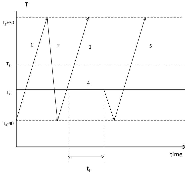
Fig. 2.1. Temperature Profile of Enthalpy Relaxation of Measurements using DSC.
