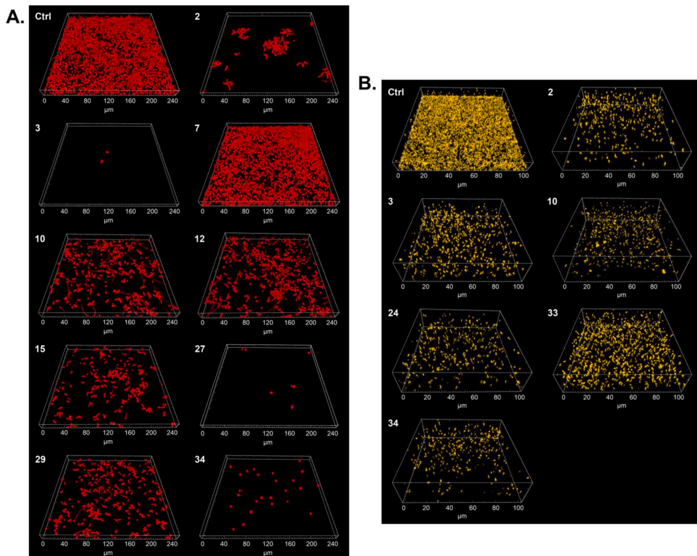
Fig. 4. Furanones with significant anti-biofilm activity as analysed by confocal laser-scanning microscopy (CLSM). (A) CLSM images of C. albicans M2396 in the presence of 2, 3, 7, 10, 12, 15, 27, 29 and 34. (B) Representative CLSM images of biofilm formed by P. aeruginosa PAO1 in the presence of 2, 3, 10, 24, 33 and 34. In both panels, control (Ctrl) represents biofilms treated with neat DMSO.
