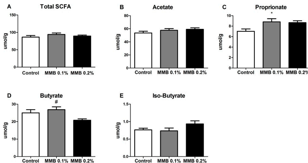
Figure 4. (A) Total short-chain fatty acid analysis, subdivided into (B) acetate; (C) propionate; (D) butyrate and (E) iso-butyrate. Data are expressed as mean \pm SEM ( n = 10 ). * p < 0.05 vs. control group, # p < 0.05 vs MMB-0.2% group.
