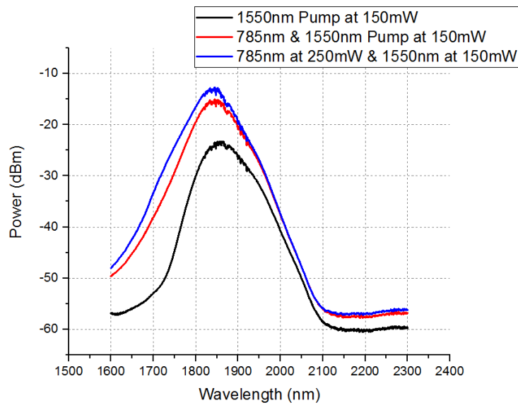
Figure 8. ASE spectra of dual and single pumped TDFAs
