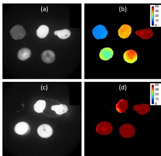
Figure 2. Images of the polymer based phosphorescent coating spotted on polyester film (spot size \sim 2-3 mm): in the oxygenated state in (a) intensity and (b) lifetime( \mu\text{s} ) scale; in the de-oxygenated state in (c) intensity and (d) PLIM ( \mu\text{s} ) mode, 22°C.
