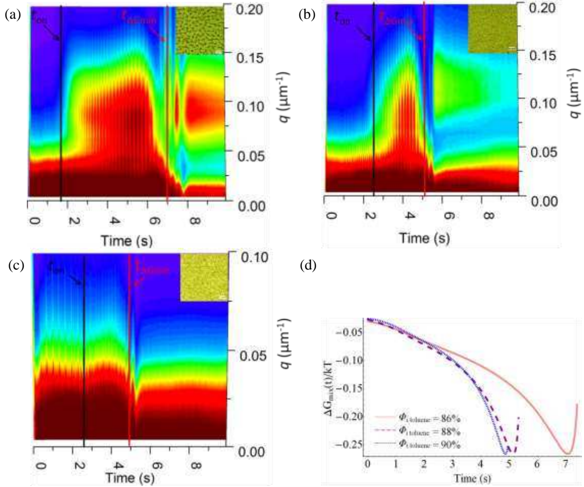
Figure 1. Off-specular scattering ( q ) for the film cast from a solution of (a) 7% PMMA, 7% PS, and 86% of toluene; (b) 6% PMMA, 6% PS, and 88% toluene; and (c) 5% PMMA, 5% PS, and 90% toluene. The insets in (a), (b), and (c) show optical images of the films (scale bars 100 \mu\text{m} ). (d) Free energy of mixing as a function of time for the film cast from solution containing 90% of toluene (dotted line), 88% of toluene (dashed line), and 86% of toluene (solid line)
