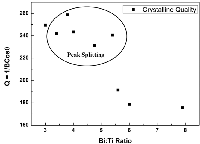
FIG. 8. The relative crystalline quality 1/(BCos\theta) plotted against Bi:Ti ratio for the second set of experiments. Points inside the circle are samples with OPBs. Here, B is peak broadening and \theta is the incident.
