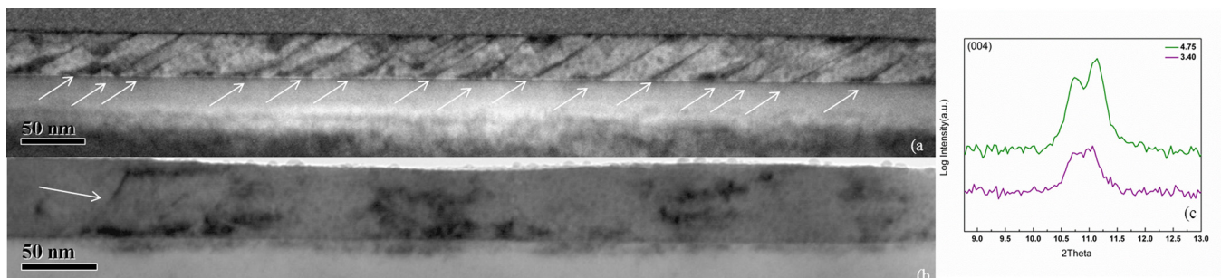
FIG. 7. Representative TEM images of BTO samples with (a) large (Bi:Ti ratio 4.75) and (b) small (Bi:Ti ratio 3.40) (c) corresponding XRD data showing extent of 2\theta splitting for the 004 reflection from each sample.
