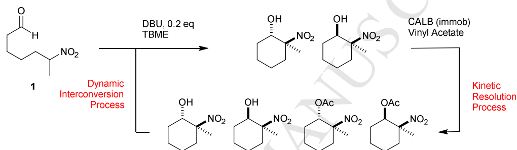
Scheme 5 Two-pot process
