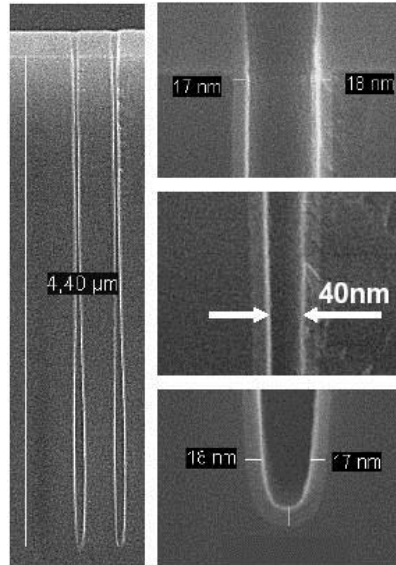
Figure 3 – A trench of aspect ratio AR~100 (4.40 \mu\text{m} deep, 40 nm wide) as required for the 90 nm ground rule in trench DRAM; the trench is evenly coated with 17-18 nm thick \text{Al}_2\text{O}_3 deposited by ALD. (image: Infineon Technologies)
