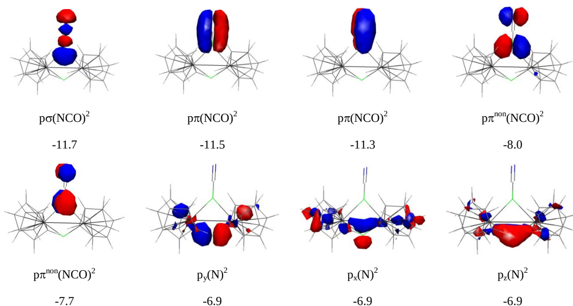
Figure 12 – Selected MOs of the product complex I3, [Hf 2 Cp 2 (NCO)(N)]. The mixing shown in I2 has allowed p\sigma(\text{NN})_2 to be polarised into p(\text{N})_2 , yielding [\text{N}]^{3-} , a net gain of one electron by that N atom. Virtual orbitals not shown: p\pi^*(\text{NCO}) , p\sigma^*(\text{NCO}) . Orbital energies in eV.
