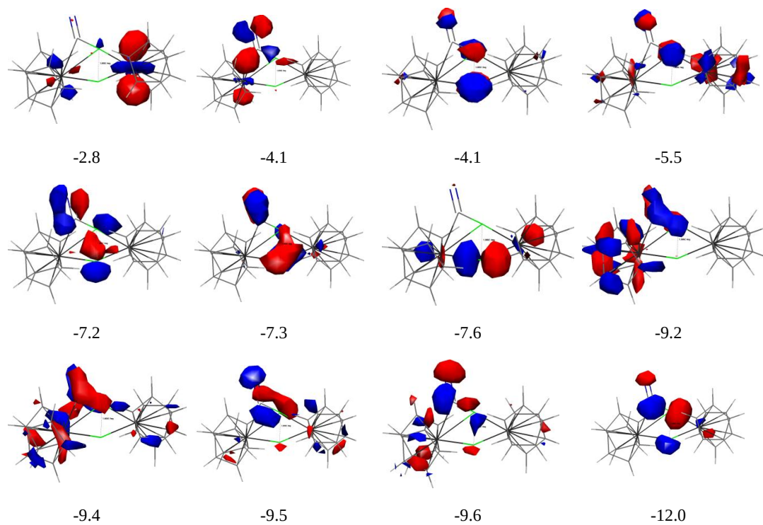
Figure 11 – Selected MOs of transition state TS2/3 linking two minima I2 and I3. We see progress in weakening of the N-N bond. Orbital energies in eV.
