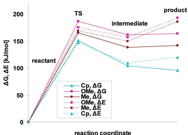
Figure 6 – Computed energetics along the decomposition pathway (Equation 1) from the data in Table 6. Lines are to guide the eye.
