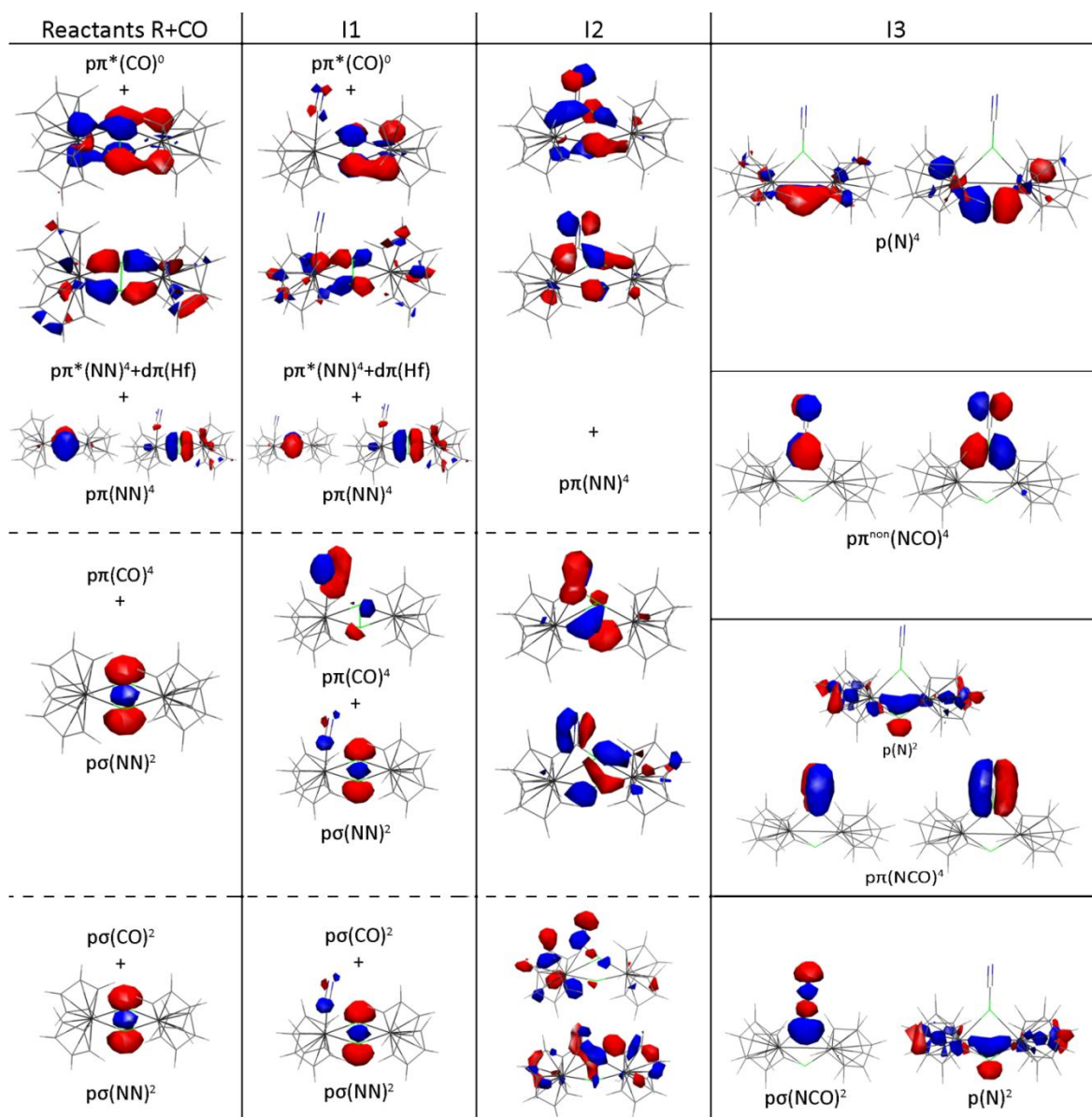
Figure 6 – How 14 of the \rho\sigma and \rho\pi electrons from CO and N 2 undergo changes in bonding during the reaction. Selected orbitals are plotted, in some cases only one of each pair of \rho\pi MOs.
