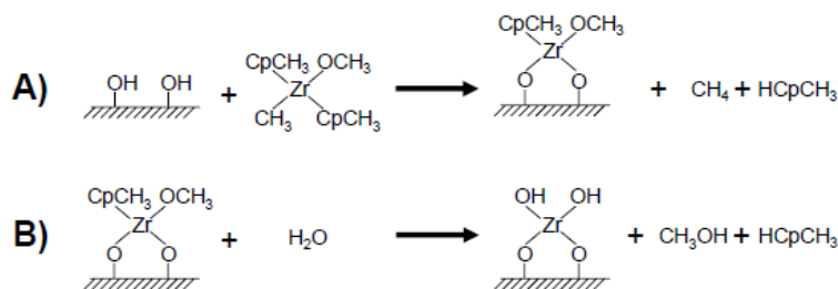
Figure 2. Illustration of proposed \text{ZrO}_2 ALD mechanism.
