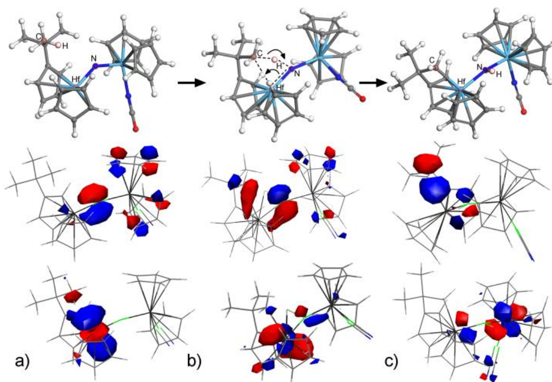
Figure 1 Computed atomic and electronic structure of (a) reactant, (b) TS and (c) product along the reaction pathway of C-H bond activation (1,2 addition of C-H bond to Hf=N bond) in model \text{Hf}_2\text{N} complexes ( \text{L}_1 = \text{C}_5\text{H}_4\text{tBu} , \text{L}_{2-4} = \text{C}_5\text{H}_5 ). First row presents structures with white = H, grey = C, pale blue = Hf, dark blue = N, red = O. The second row presents isosurface plots of high-lying M:d-derived orbitals: (a) HOMO-1 of reactant, (b) HOMO-1 of TS and (c) HOMO of product. The third row presents: (a) LUMO of reactant (b) LUMO of TS (c) LUMO of product along the same reaction pathway.
