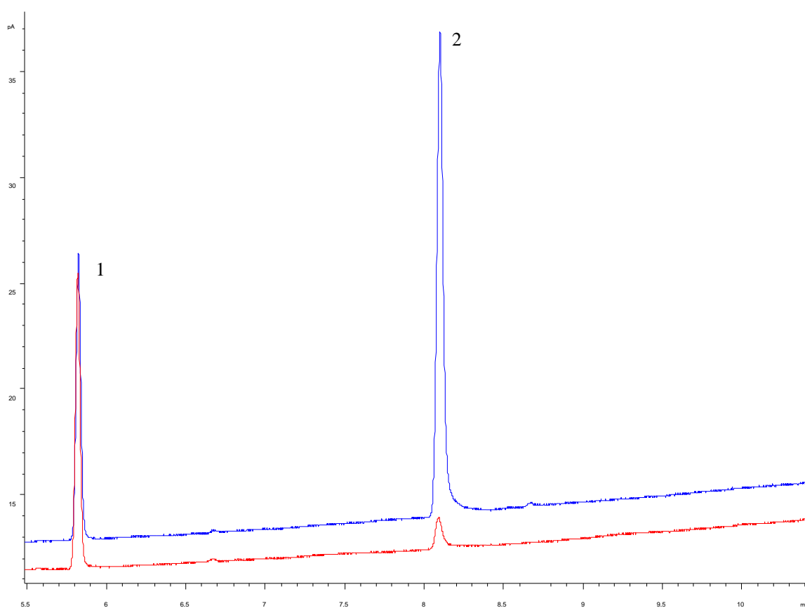
Figure 1. Cholesterol profile by gas chromatography with flame ionization detector in control cheese and experimental cheese with 1% of beta cyclodextrin. Peaks: 1 = 5\alpha -cholestane; 2 = cholesterol. Blue line: control cheese (CC); Red line: experimental cheese (EC).
