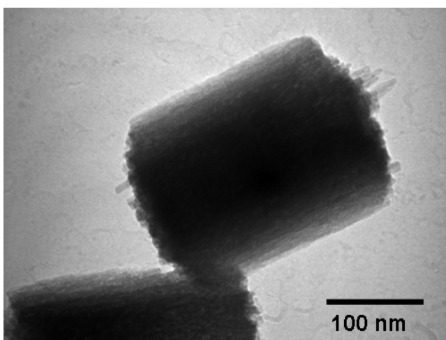
Fig. 4. TEM of individual Pt nanowire following dissolution of alumina membrane with CNT protrusions evident at both ends.
