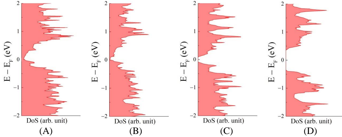
Fig. S3 – The density of states for bismuth bulk and thin films from DFT calculations corresponding to schematic band structures shown in Fig. 3 of the main text for simulation slabs of thickness (A) bulk, (B) 8 nm, (C) 4 nm, and (D) 1.5 nm with hydroxyl termination.
