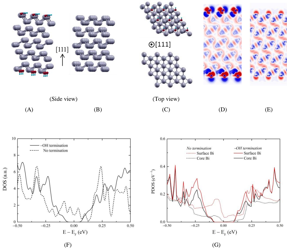
Fig. S2 - Atomic illustration of relaxed (strain free) Bi slab models. Side view (A) with hydroxyl surface termination, and (B) without surface termination. Top view with hydroxyl (C-top) and without (C-bottom). Contour plot of lateral plane charge difference density distributions for Bi slabs for (D) hydroxyl surface termination, and (E) without. (F) Total DoS for the Bi thin films with -OH termination and without. (G) PDoS for surface and core Bi atoms with and without -OH termination.
