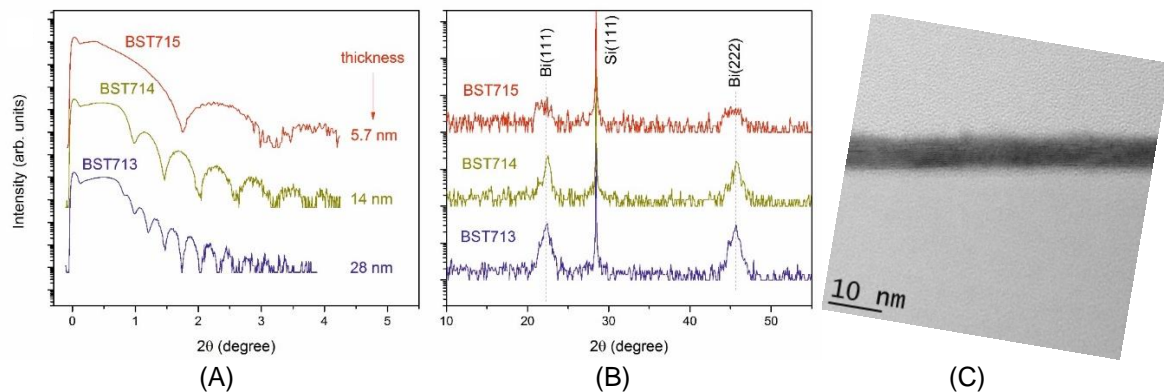
Fig. S1 - (A) XRR of bismuth film with thicknesses of 5.7 nm, 14 nm and 28 nm on Si (111). (B) XRD of 5.7 nm, 14 nm and 28 nm bismuth film thicknesses on Si (111). (C) HR-XTEM of 5.7 nm Bi film grown by MBE on Si(111).
