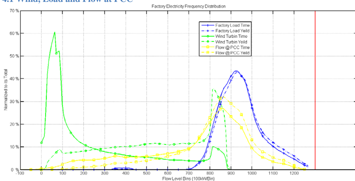
Figure 6. Frequency distribution showing wind, load and flow at the PCC.
