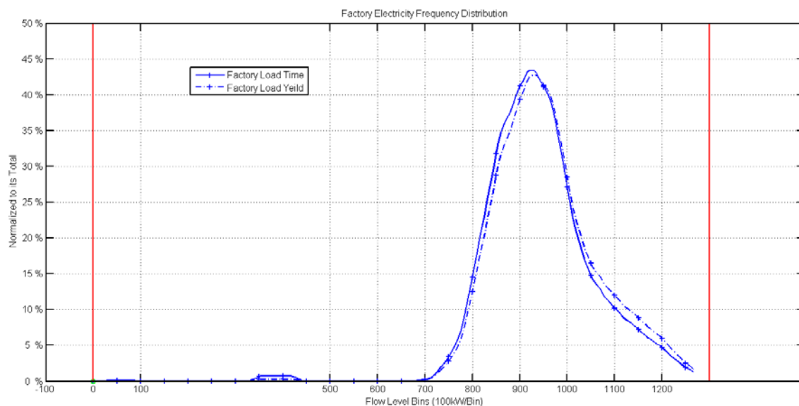
Figure 5. Frequency distribution of site electrical flow at the PCC.
