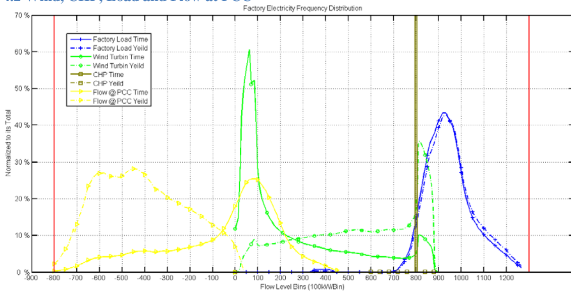
Figure 7. Frequency distributions of CHP generation, wind generation, load and flow at the PCC.
