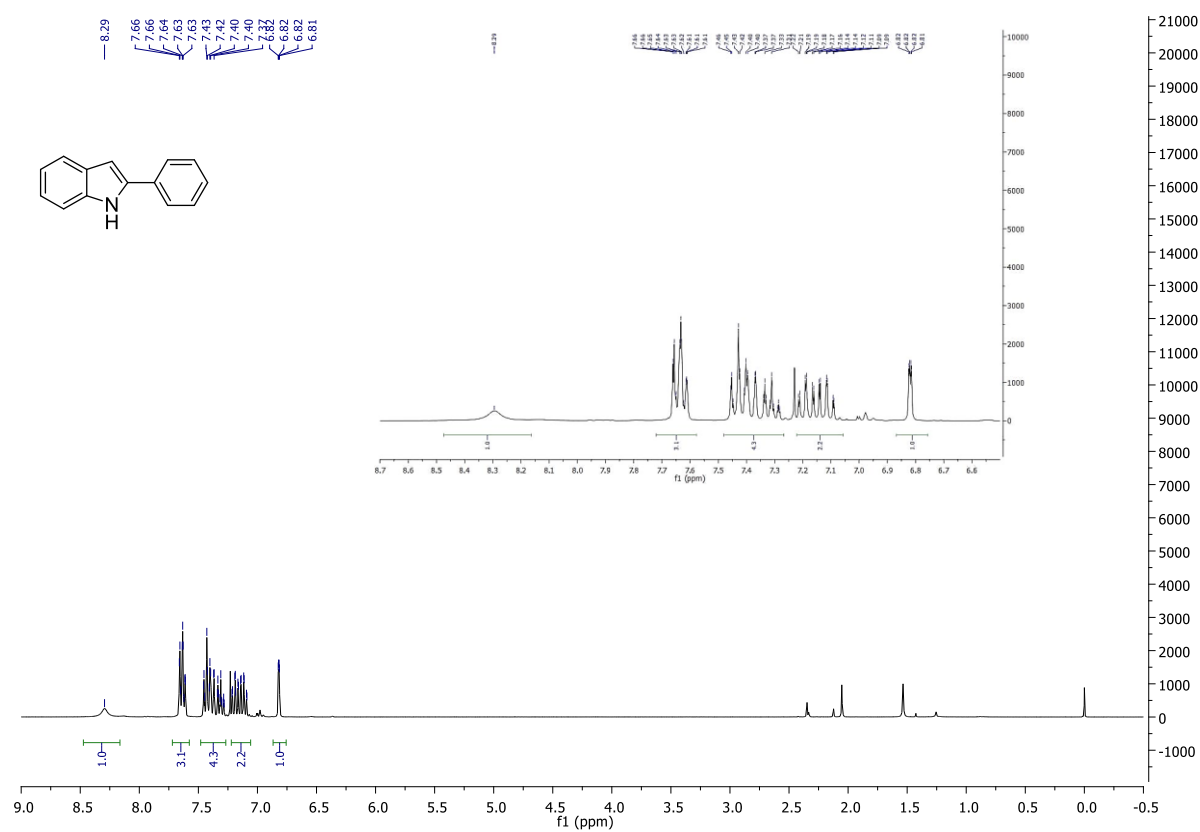
Figure S3. 1 H NMR spectrum (CDCl 3 , 300 MHz) of 2-phenylindole.
