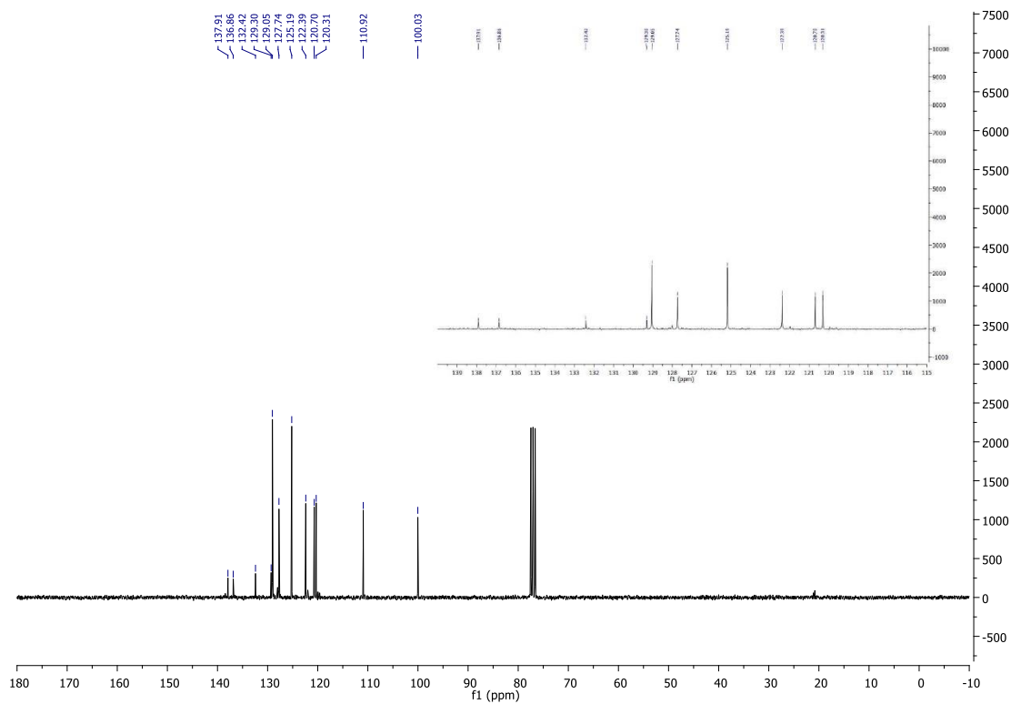
Figure S4. 13 C NMR spectrum (CDCl 3 , 75 MHz) of 2-phenylindole.
