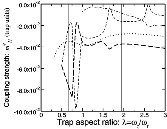
FIG. 3. Coupling strength m_{ij} from the m=0 quadrupole state for C=1000 as a function of trap aspect ratio \lambda : coupling to the (+) hybrid mode (short-dashed line), to the (-) hybrid mode (long-dashed line), and to the n=1, l=2 state (dot-dashed line). The hydrodynamic calculation for the breather mode [9] is shown as the dotted line. Second-harmonic resonance for the (+) hybrid mode occurs near \lambda=0.68 and \lambda=1.95 according to hydrodynamic theory [8] and Fig. 1, as indicated by the vertical lines.
