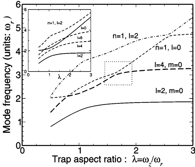
FIG. 1. Frequencies of the the four lowest even-parity m=0 excitations in units of the radial trap frequency \omega_r . Present Bogoliubov theory for N=4650 atoms ( C=1000 ) is compared with hydrodynamic predictions (inset) ( C \rightarrow \infty ). The labeling of the curves in the main graph corresponds to the quantum numbers for a spherical trap: \lambda=1 . The (+) hybrid mode is marked by the short-dashed line, and the (-) hybrid by the long-dashed line. The pump mode ( l=2, m=0 ) is the solid line. Hybridization of the Bogoliubov l=0 mode occurs near \lambda=0.80, 1.63 , and 2.60 . Second-harmonic resonance between the pump and (+) hybrid occurs at \lambda=1.989 .
