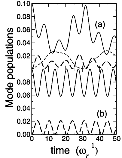
FIG. 4. Mode conversion for C=1000 and 10% pump population. (a) \lambda=2.00 : population of fundamental ( n=0, l=2, m=0 ) quadrupole mode (full line); population of the off-resonant (-) mode ( n=0, l=4, m=0 ) (long-dashed line); population of resonant second-harmonic (+) mode n=1, l=0, m=0 (short-dashed line). (b) Mode conversion for \lambda=1.65 . The (+) dark-state hybrid has negligible conversion: population of fundamental (quadrupole) mode (full line); population of (+) dark-state hybrid (short-dashed line); population of (-) hybrid (long-dashed line).
