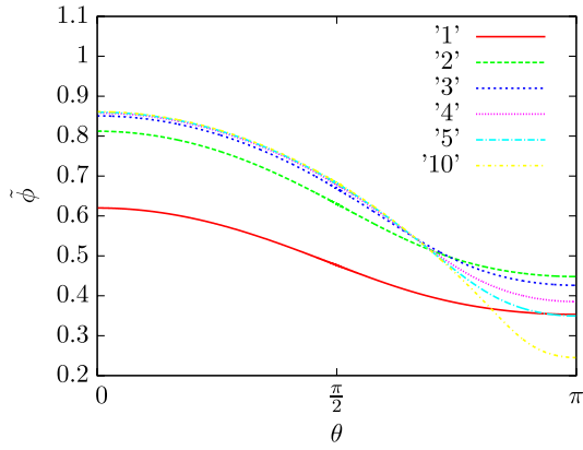
FIG. 3 (color online). \hat{\phi} on S^3 with \beta = 10 .
