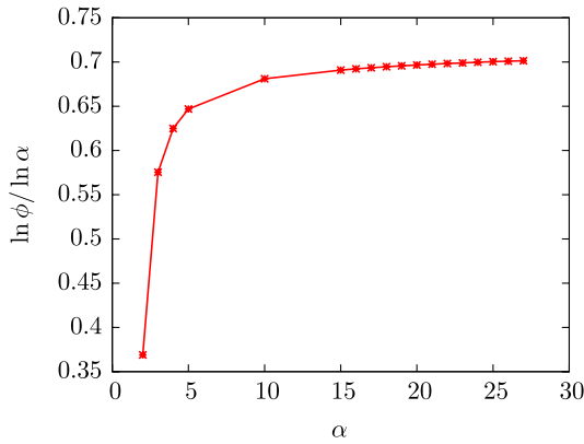
FIG. 4 (color online). \ln \phi / \ln \alpha vs \alpha for \beta = 7 .
