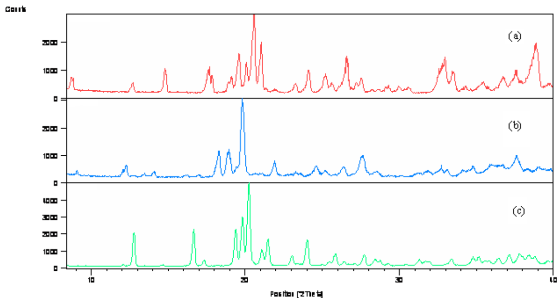
Figure 4. PXR D patterns of (a) 1-deoxy-D-lactose, 4 (b) \alpha\beta -D-lactose and (c) \alpha -D-lactose monohydrate.
