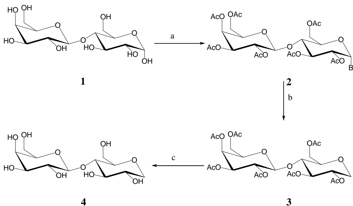
Scheme 1. Preparation of 1-deoxy-D-lactose: (a) 25 AcBr/AcOH, room temperature, 1hr, 100%; (b) \text{Bu}_3\text{SnH} , AIBN, MeOH, 67°C, 1hr, 67%; (c) KOMe/MeOH, 1hr, 54%.
