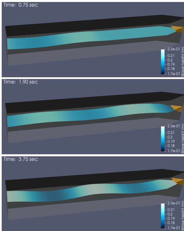
Fig. 4. Snapshots of the numerically computed free surface h(x, y, t) = \bar{H}(x, y) + \eta(x, y, t) (colour denotes height in meters, with initial still water level H_0 = 0.2\text{m} ), as it evolves in the wavetank with V-shaped contraction (times shown on the pictures). The buoy resides in the corner of the contraction and is shown using orange colour.
