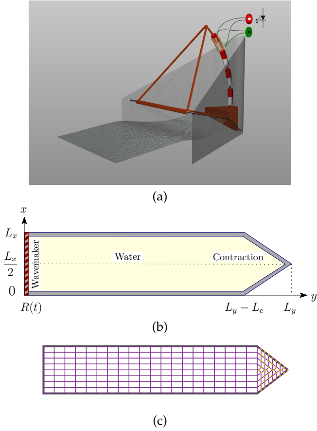
Fig. 2. (a) Sketch of our wave-energy device with its horizontal axle at the contraction entrance, and its three-dimensional tetrahedral buoy in the corner of the contraction. The buoy is attached to an induction motor, consisting of magnets on the arc moving through the hollow cylindrical coils indicated in yellow, while the LEDs are shown with green and red. (b) Top-view schematic of the wave-energy tank used in the simulations, and (c) the finite-element mesh.
