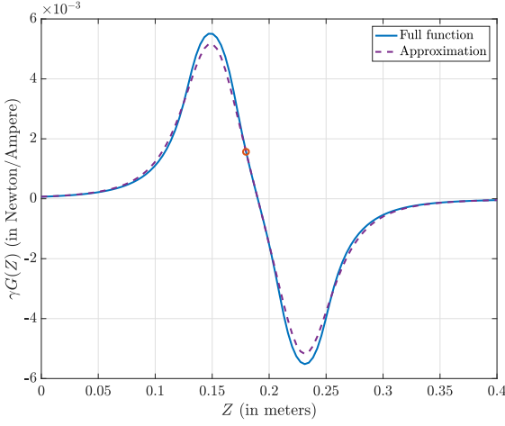
Fig. 3. Function G(Z) (defined in (5)) and its approximation G_{\text{approx}}(Z) in the far field of the magnet (defined in (6)). The circle denotes the value G(Z) at the rest position \bar{Z} = 0.18 . The values used for the rest of the parameters are taken from the table found in the appendix of [2].
