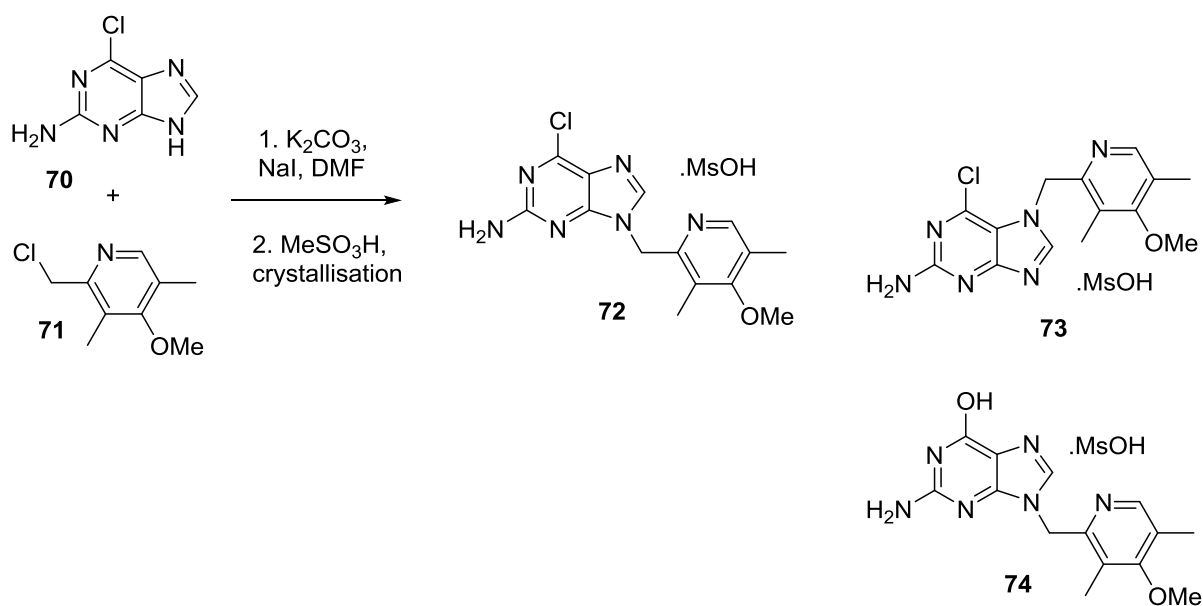
Scheme 19. Route to HSP90 Inhibitor
