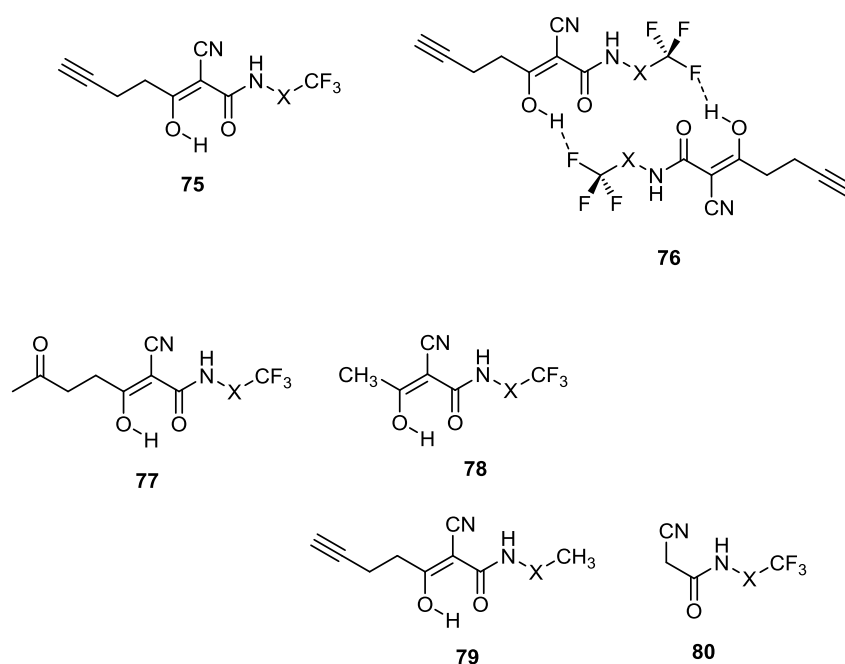
Figure 5. API 'X' and Impurities
