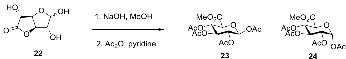
Scheme 5. Preparation of Methyl Tetra- O -acetyl-D-glucopyranuronate
