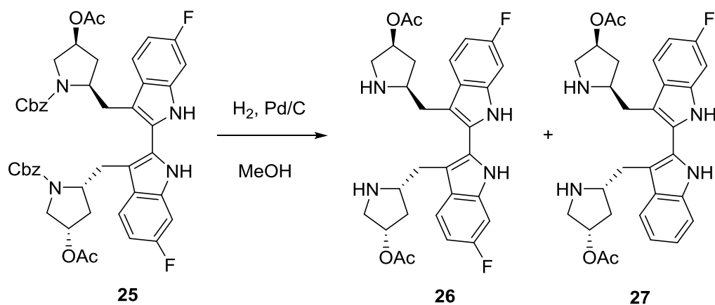
Scheme 6. Deprotection by Hydrogenation Step in a Route to Birinapant
