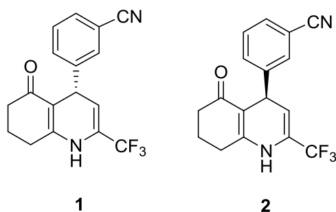
Figure 1. ZD0947 and Enantiomer
