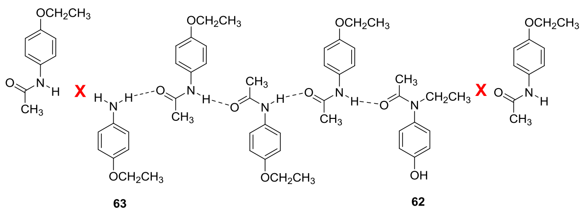
Scheme 16. Likely Discontinuity of the Phenacetin Amide C4 Chain by 4-Hydroxy-N-ethylacetanilide 62 and 4-Ethoxyaniline 63
