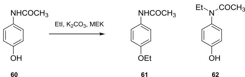
Scheme 15. Preparation of Phenacetin
