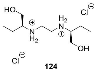
Figure 19. Ethambutol Dihydrochloride
